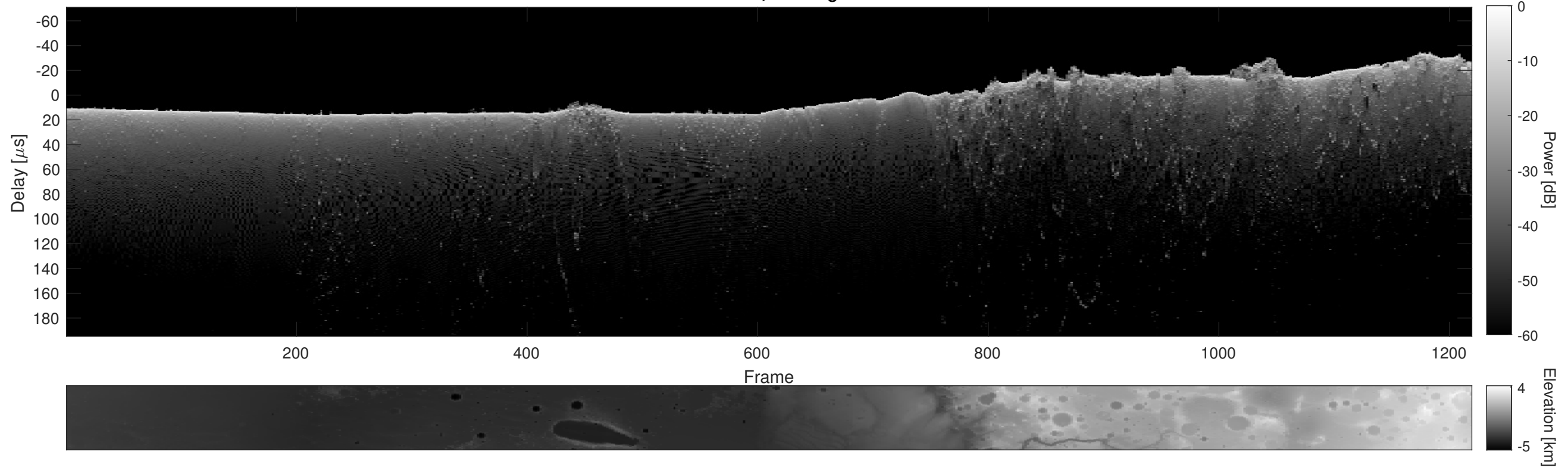
Orbit 11366, Cluttergram
