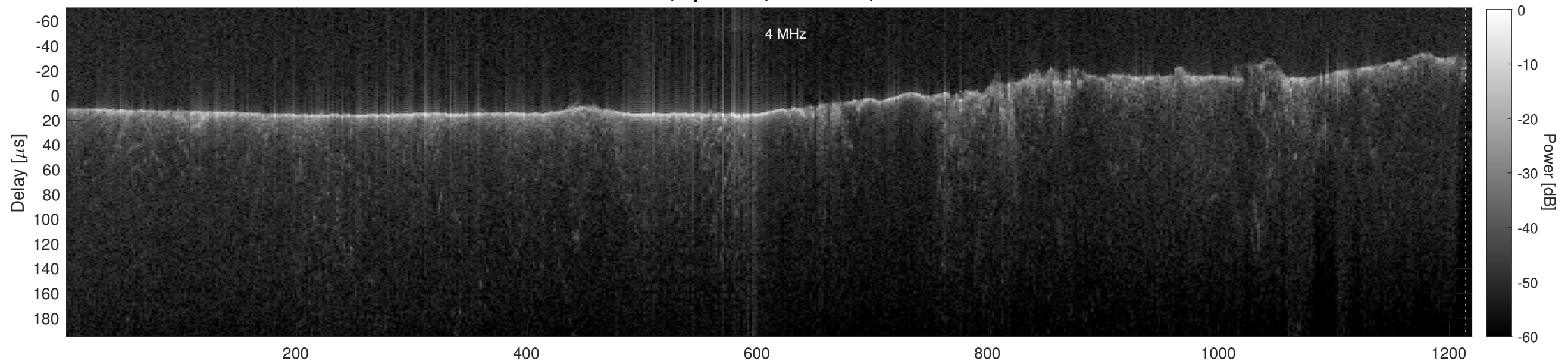
Orbit 11366, Cluttergram
