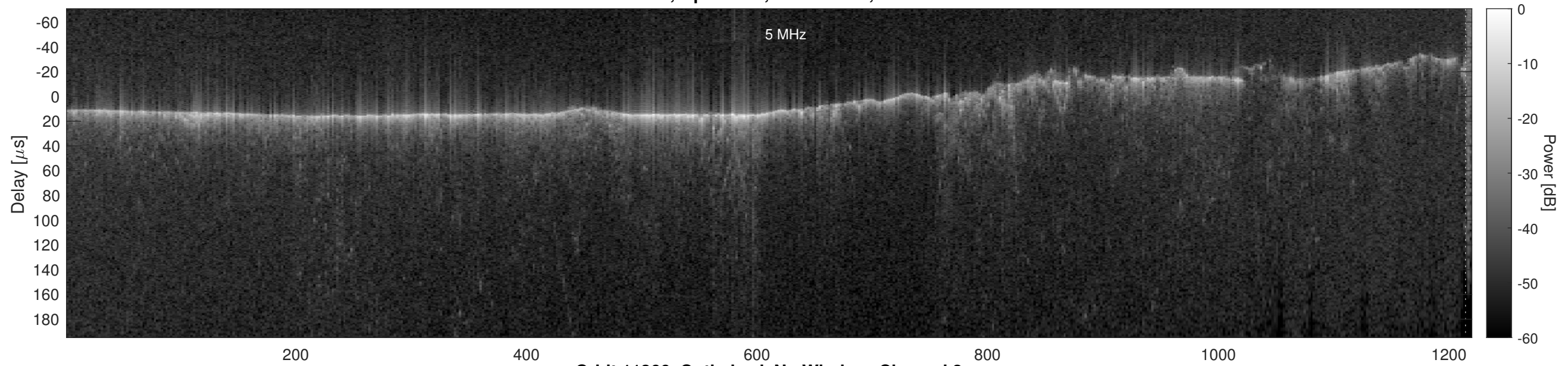
Orbit 11366, Optimized, No Window, Channel 2
