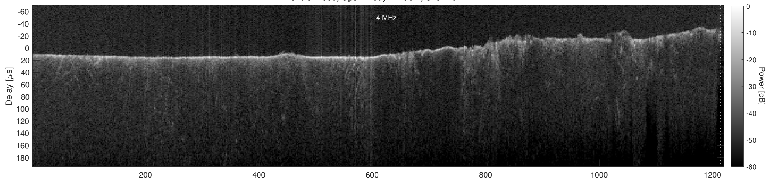
Orbit 11366, Cluttergram
