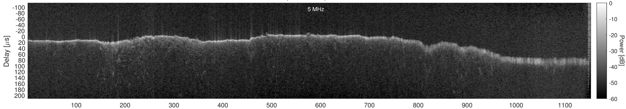
Orbit 11367, Window, Channel 1, Chapman
