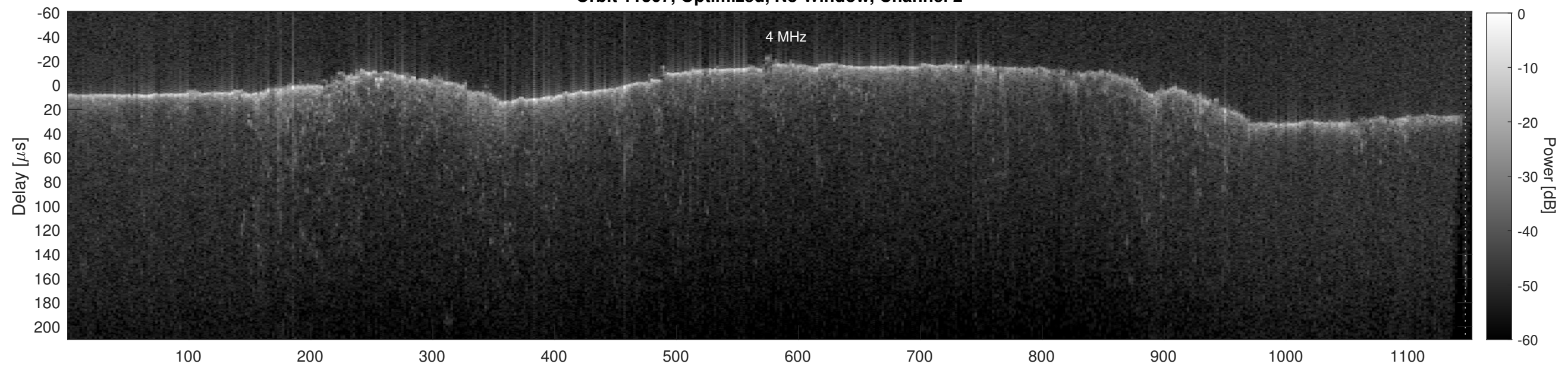
Orbit 11367, Cluttergram
