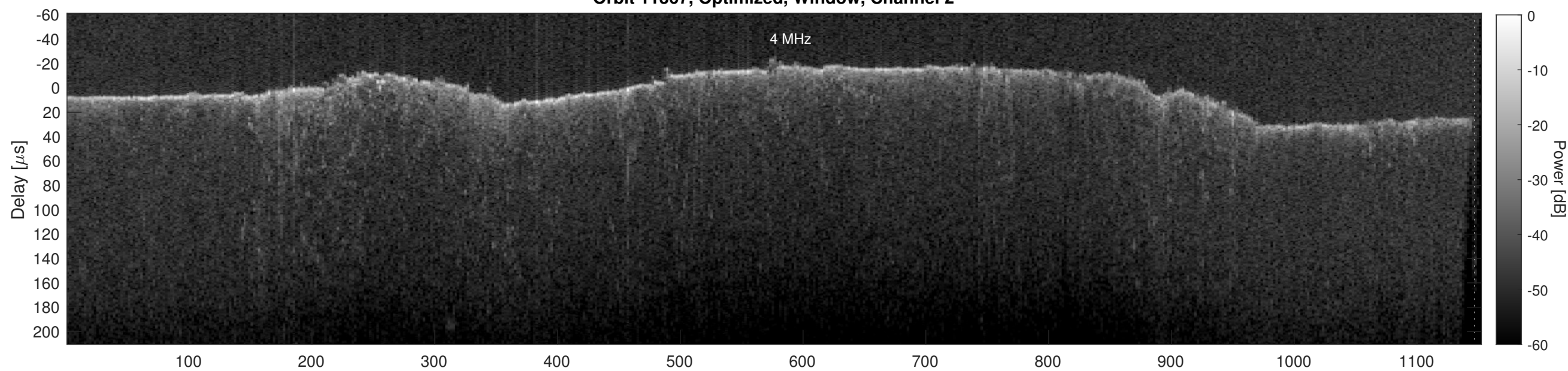
Orbit 11367, Cluttergram
