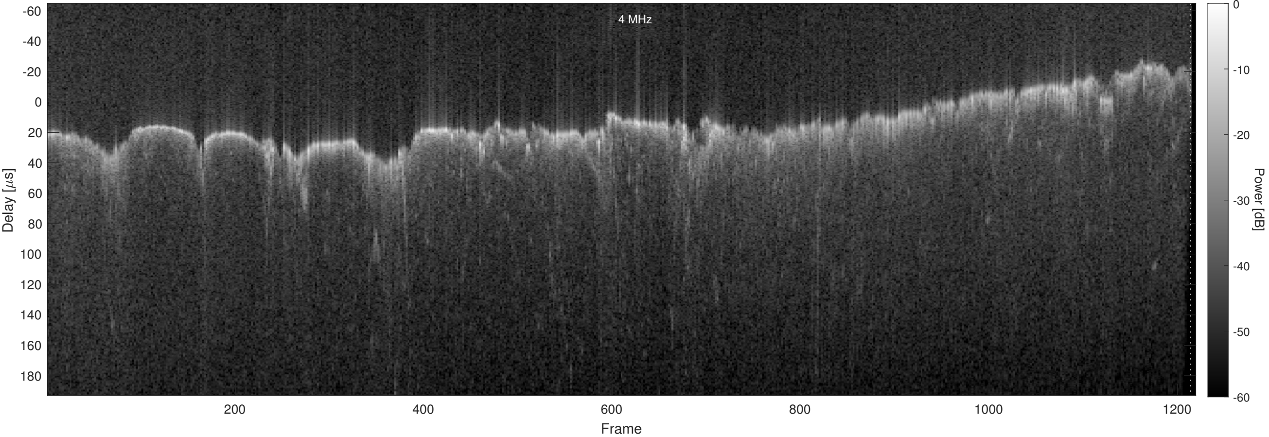
Orbit 11368, Chapman, No Window, Channel 2
