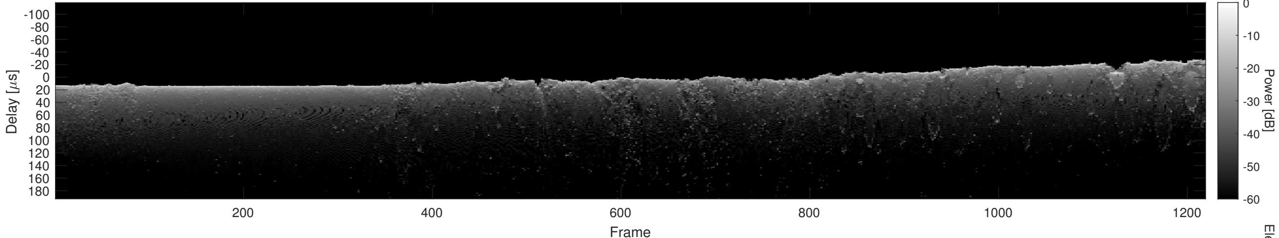
Orbit 11368, Cluttergram
