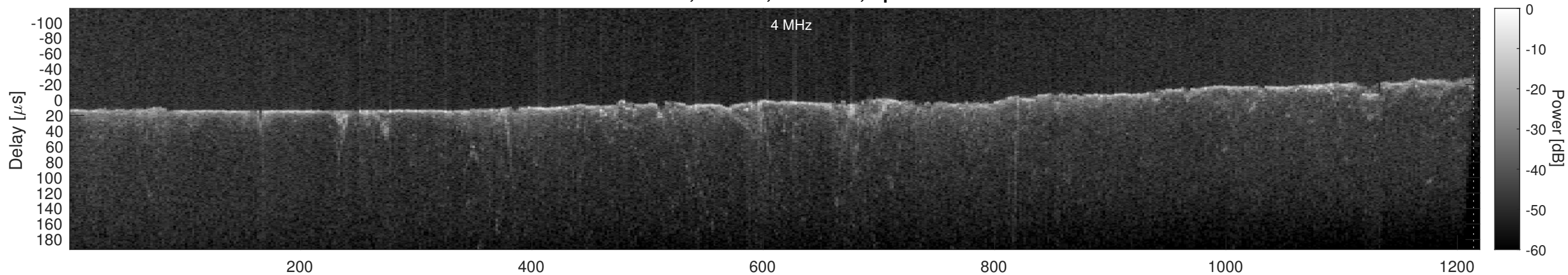
Orbit 11368, Cluttergram
