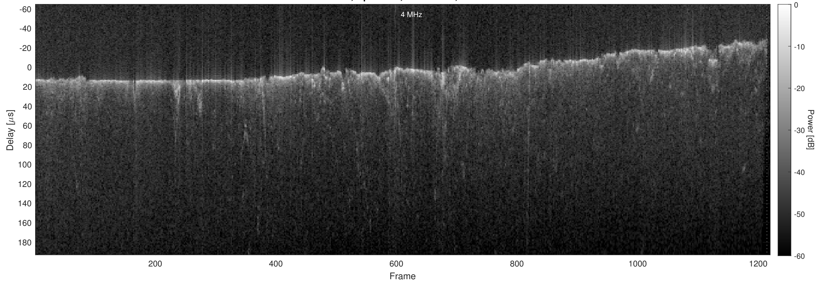
Orbit 11368, Optimized, No Window, Channel 2
