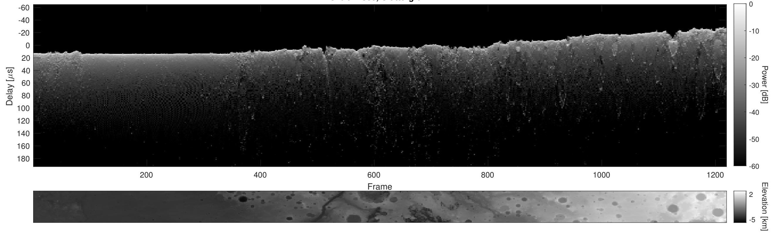
Orbit 11368, Cluttergram
