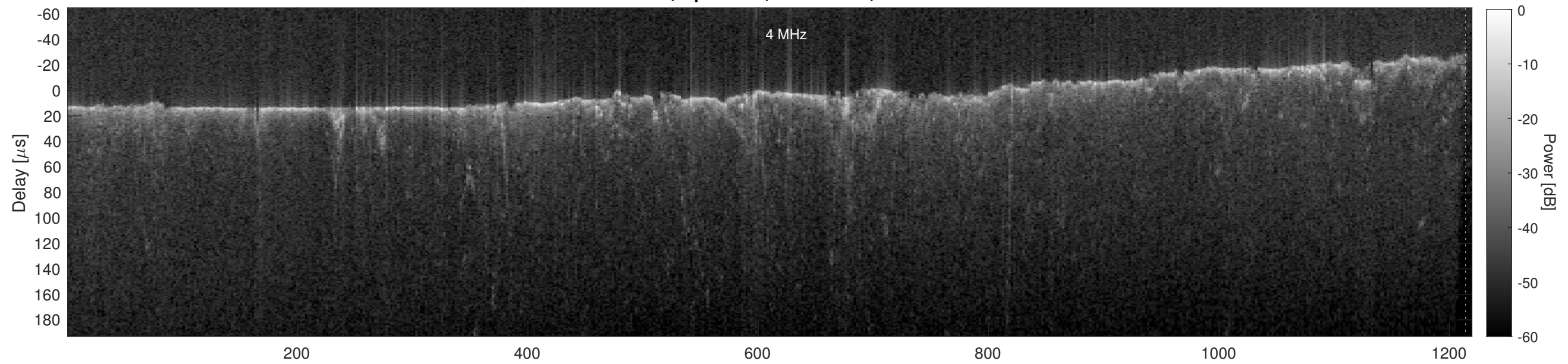
Orbit 11368, Cluttergram
