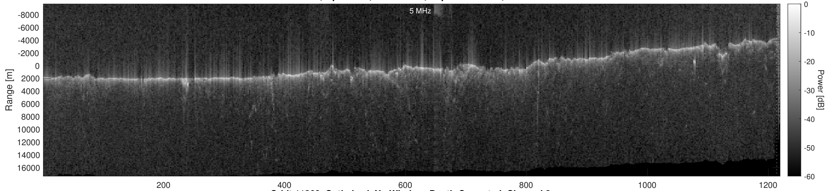
Orbit 11368, Optimized, No Window, Depth-Corrected, Channel 2
