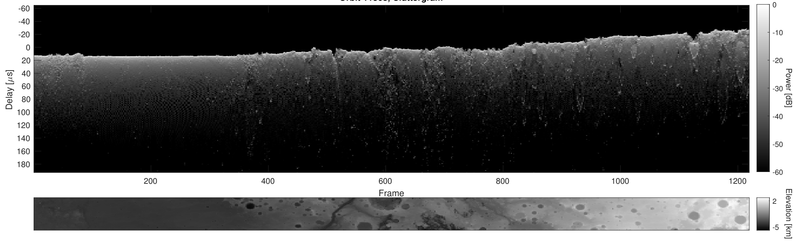
Orbit 11368, Cluttergram
