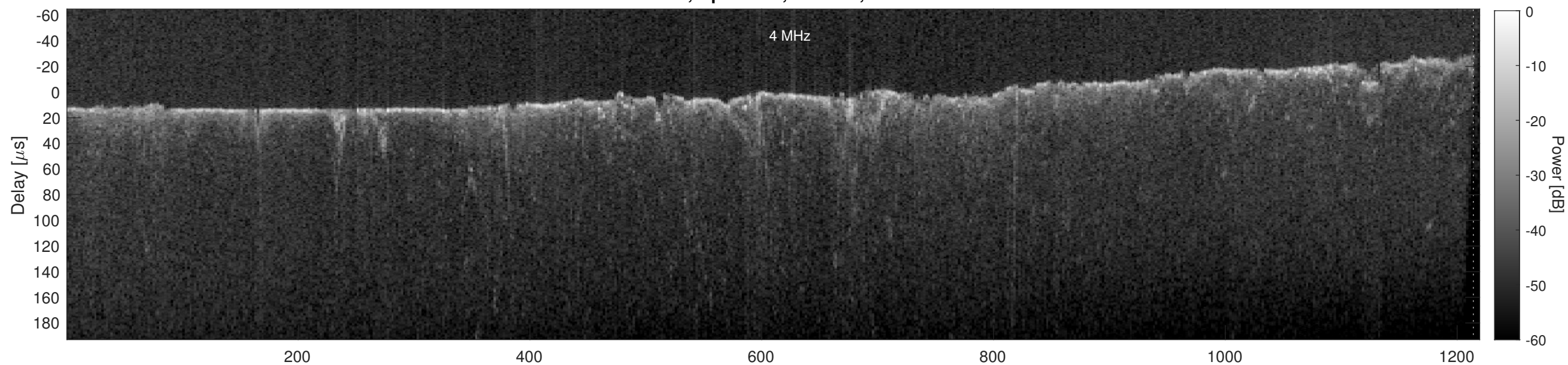
Orbit 11368, Cluttergram
