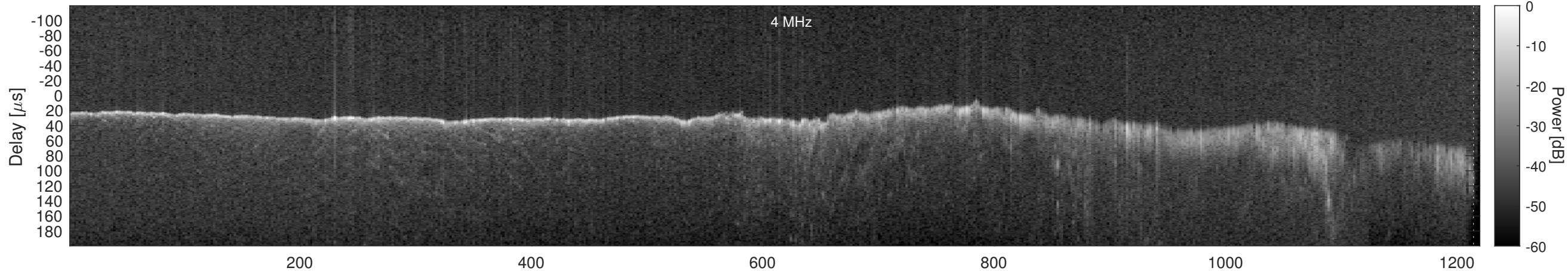
Orbit 11370, Window, Channel 2, Chapman
