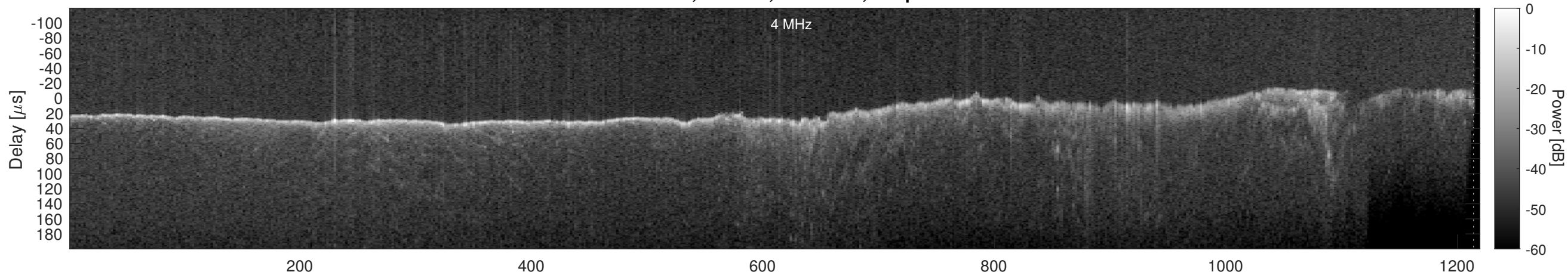
Orbit 11370, Window, Channel 2, Optimized
