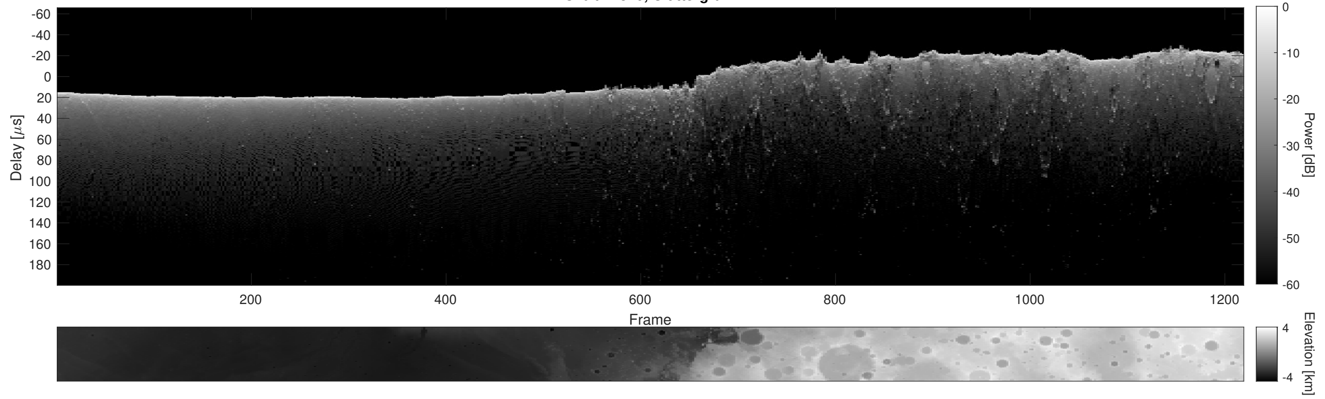
Orbit 11370, Cluttergram
