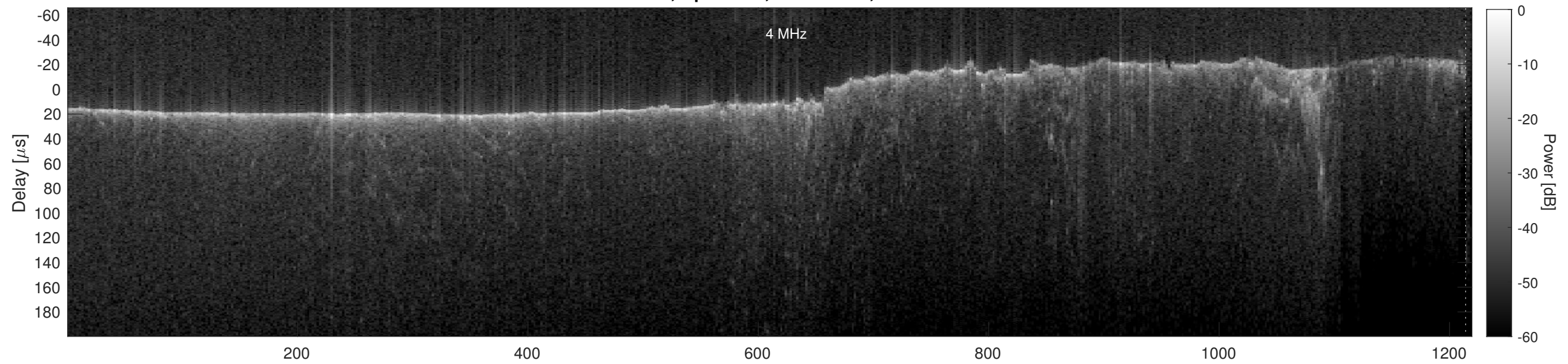
Orbit 11370, Cluttergram
