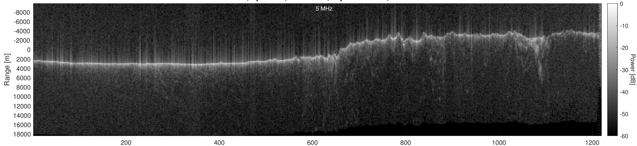
Orbit 11370, Optimized, No Window, Depth-Corrected, Channel 2
