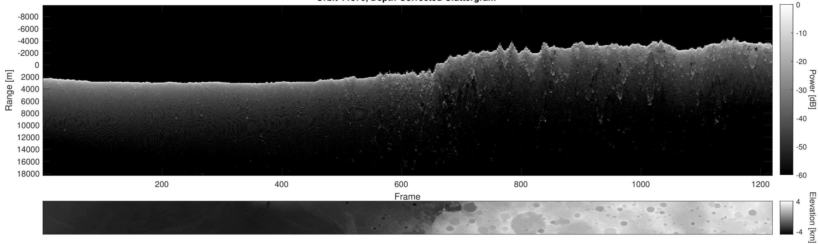
Orbit 11370, Depth-Corrected Cluttergram
