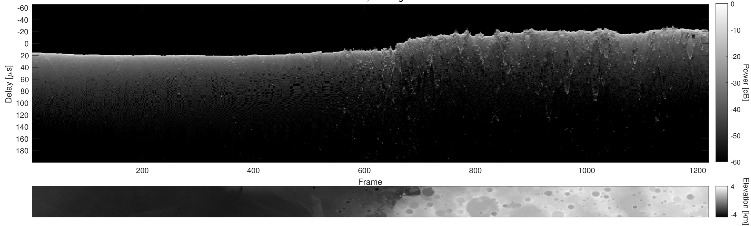
Orbit 11370, Cluttergram
