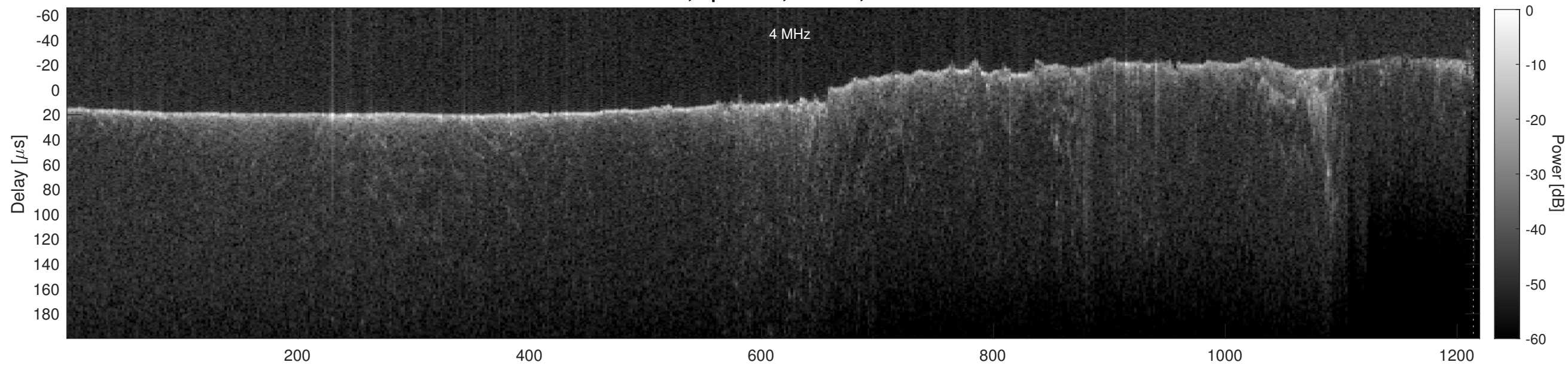
Orbit 11370, Cluttergram
