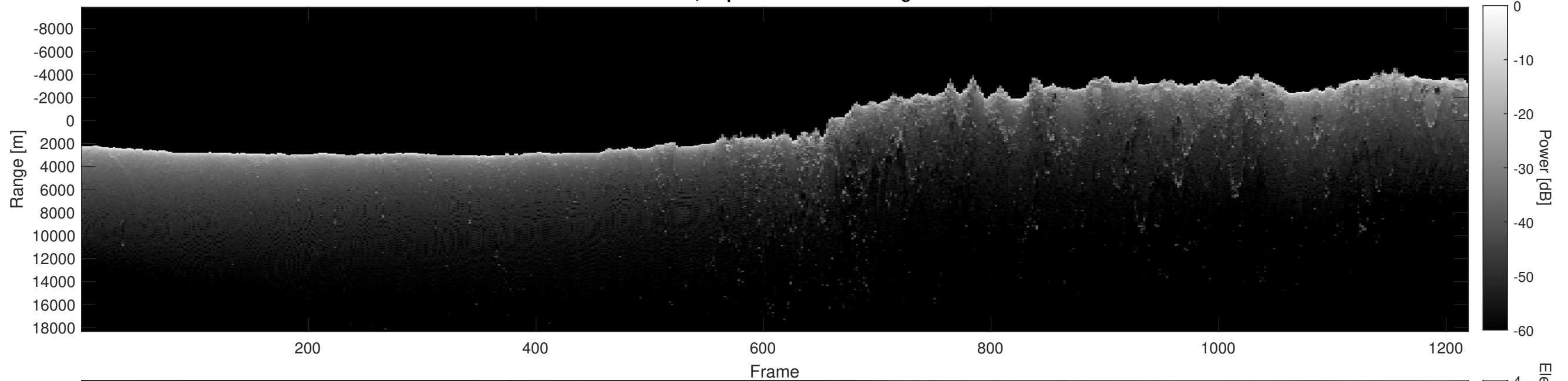
Orbit 11370, Depth-Corrected Cluttergram
