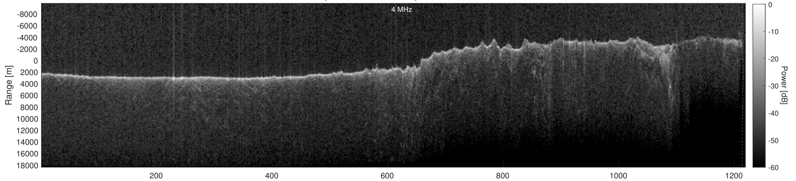
Orbit 11370, Depth-Corrected Cluttergram
