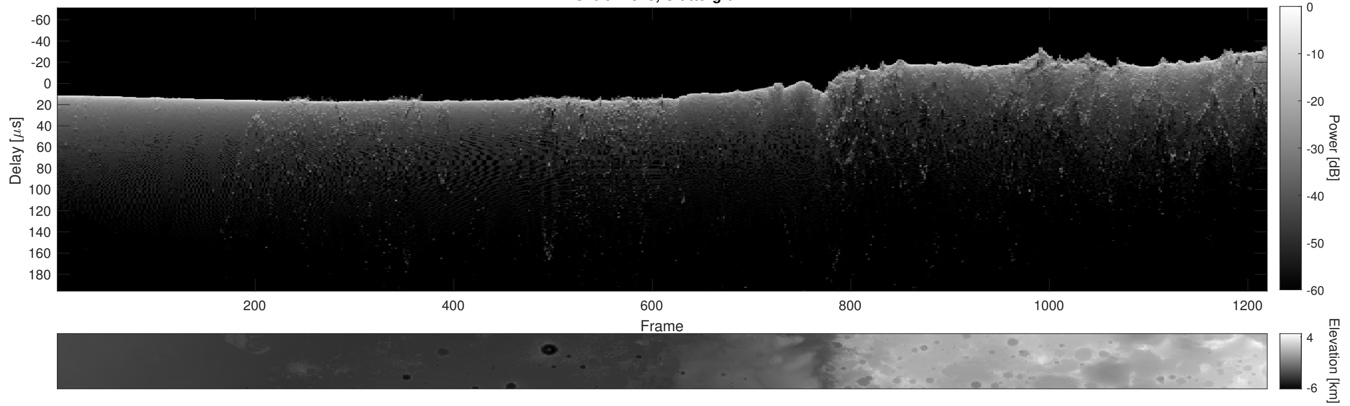
Orbit 11373, Cluttergram
