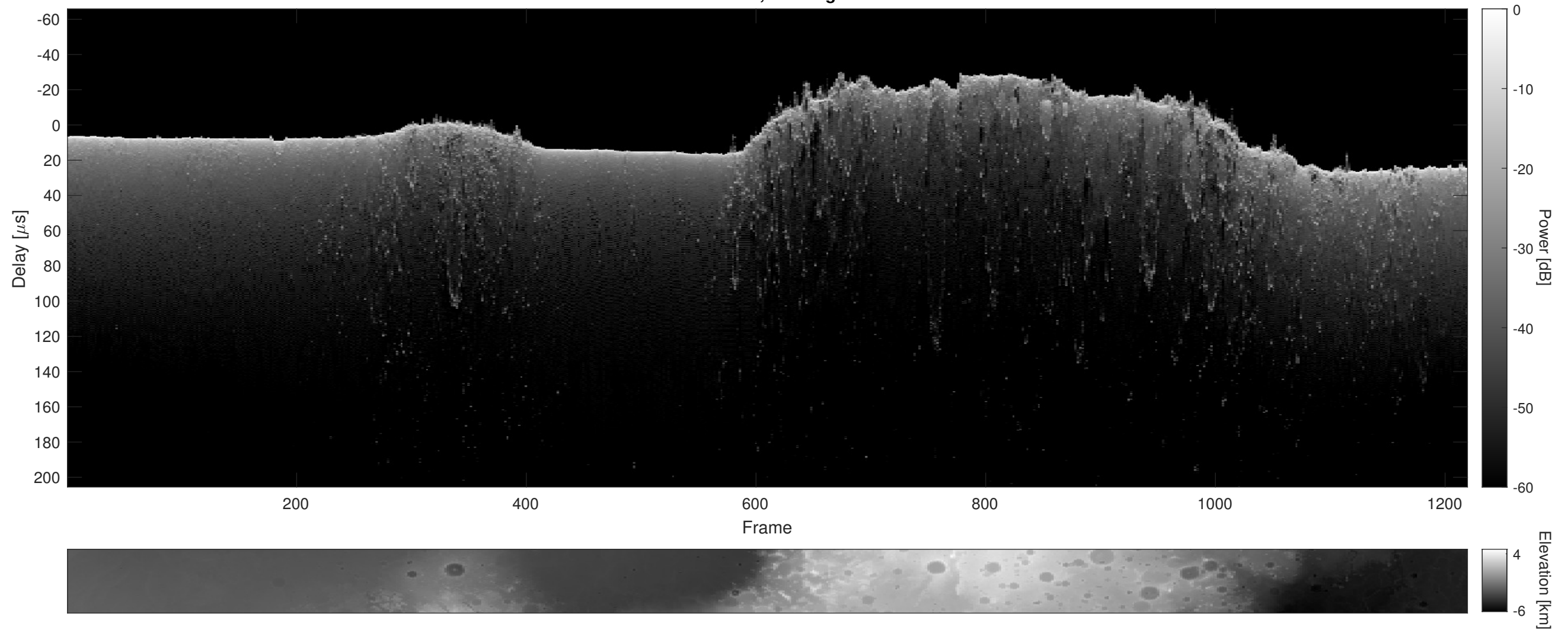
Orbit 11374, Cluttergram
