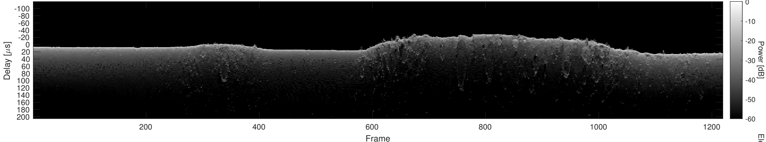
Orbit 11374, Cluttergram
