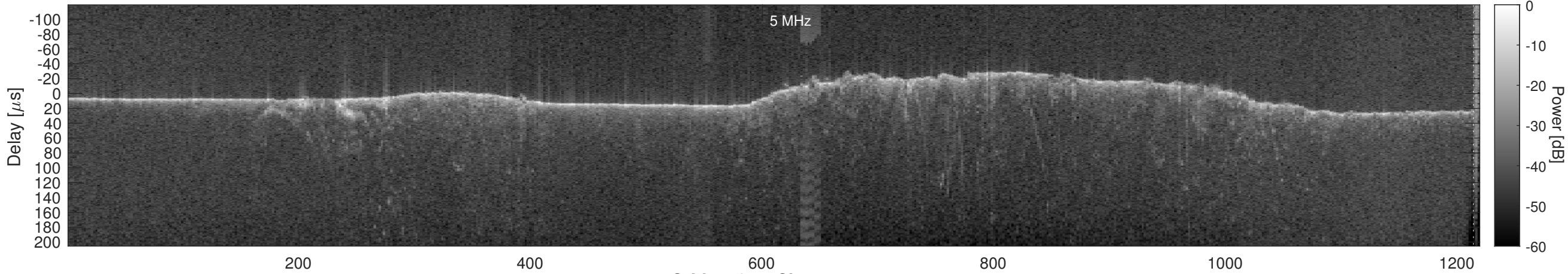
Orbit 11374, Cluttergram
