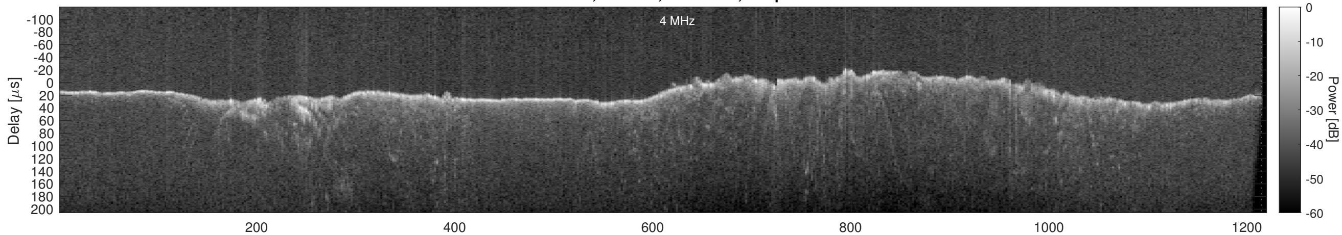
Orbit 11374, Window, Channel 2, Optimized
