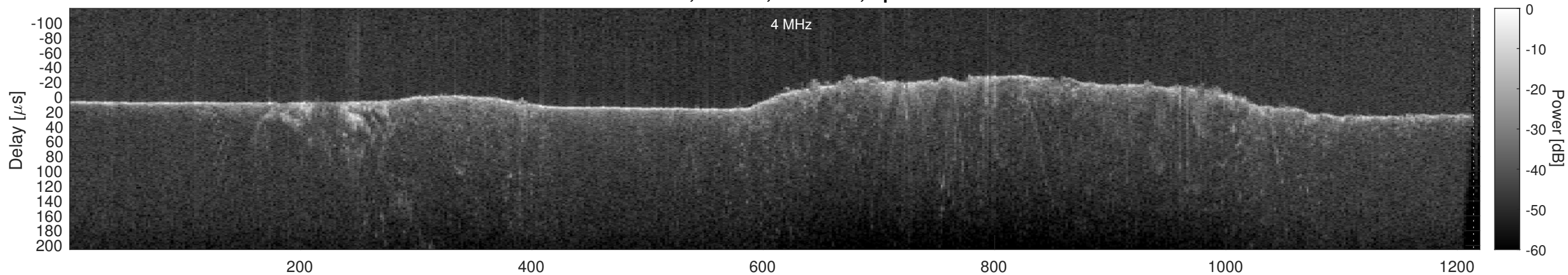
Orbit 11374, Cluttergram
