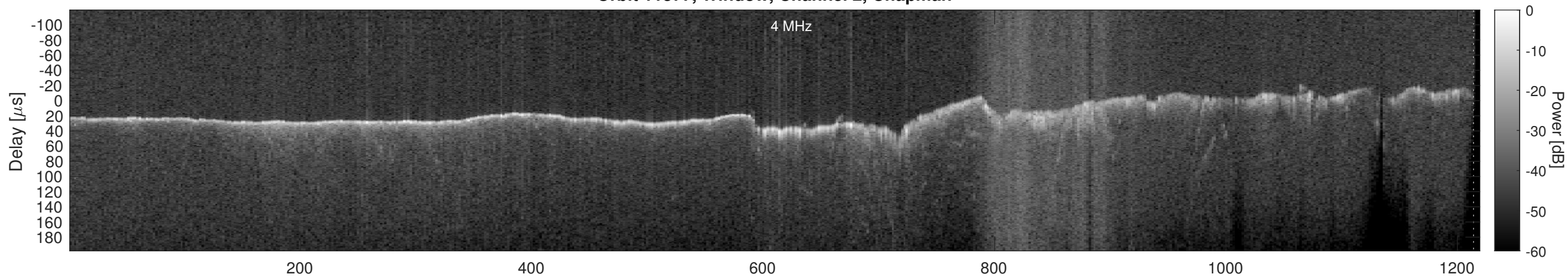
Orbit 11377, Window, Channel 2, Optimized
