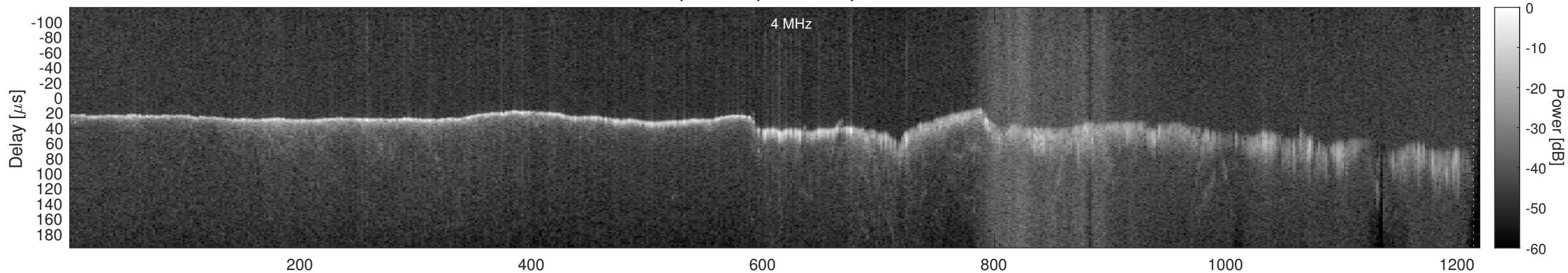
Orbit 11377, Window, Channel 2, Chapman
