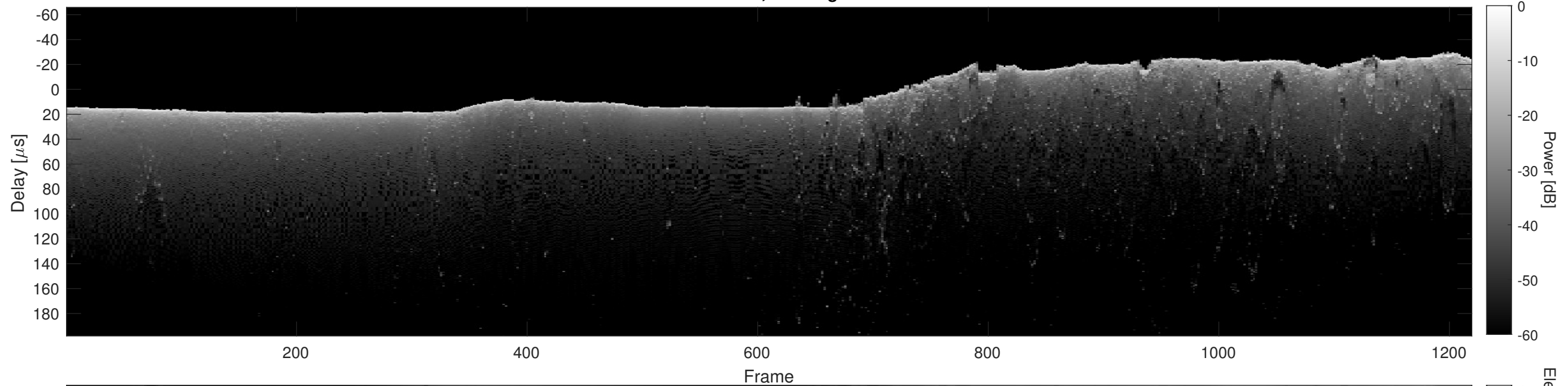
Orbit 11377, Cluttergram
