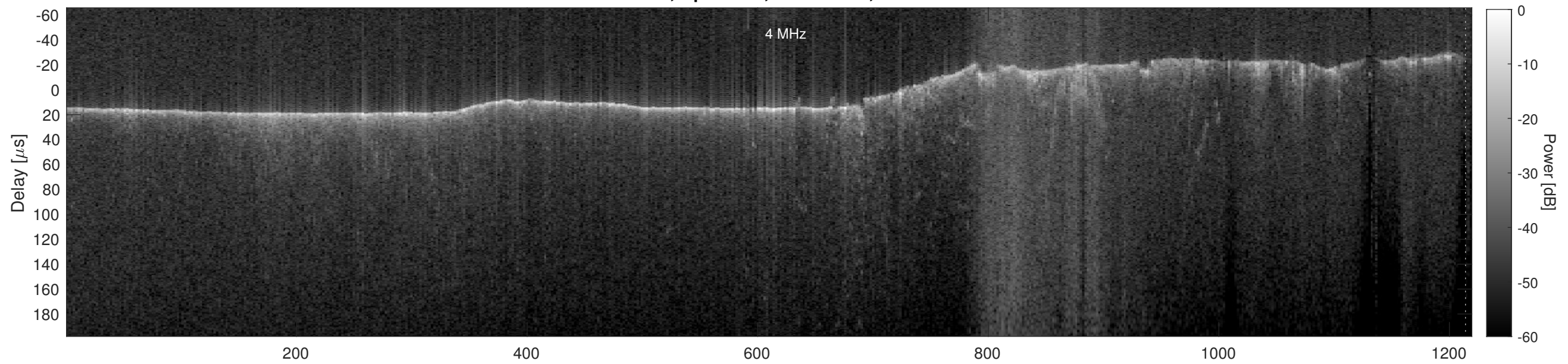
Orbit 11377, Cluttergram
