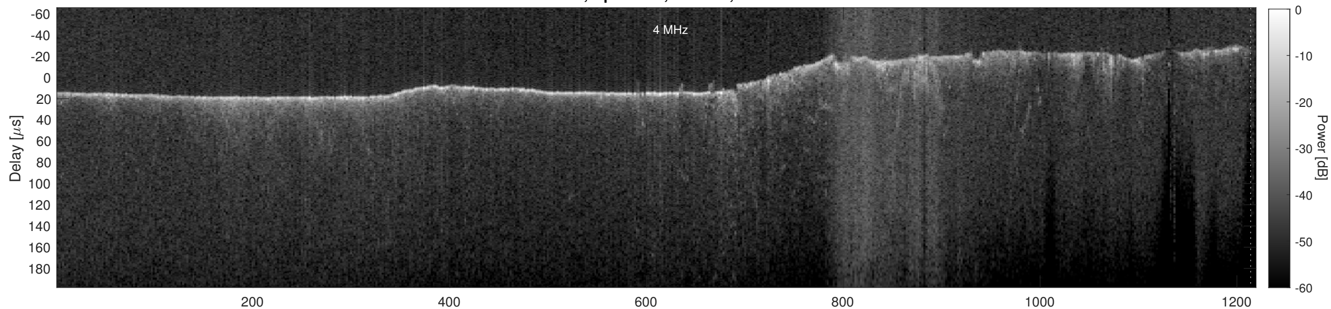
Orbit 11377, Cluttergram
