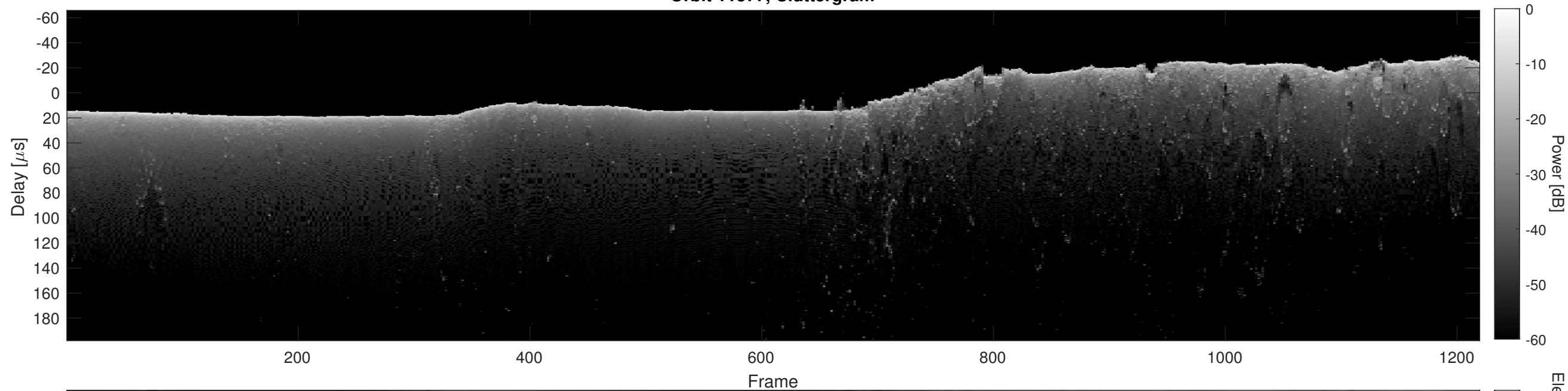
Orbit 11377, Cluttergram
