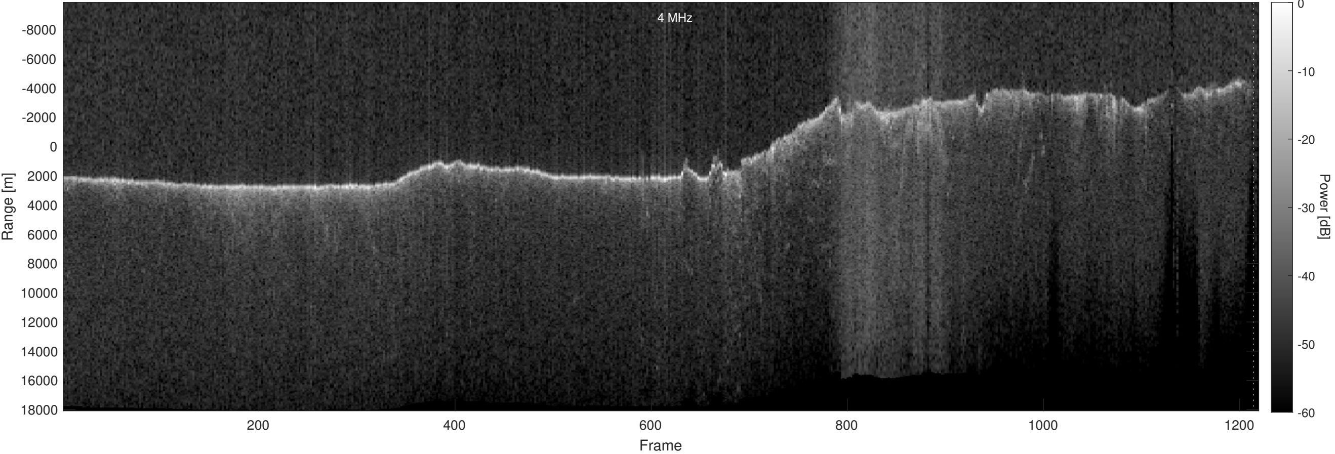
Orbit 11377, Optimized, Window, Depth-Corrected, Channel 2
