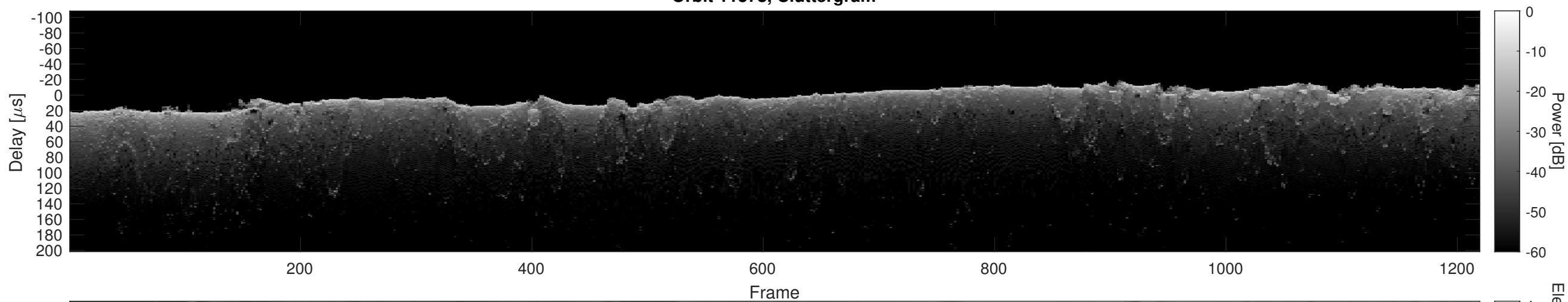
Orbit 11378, Cluttergram
