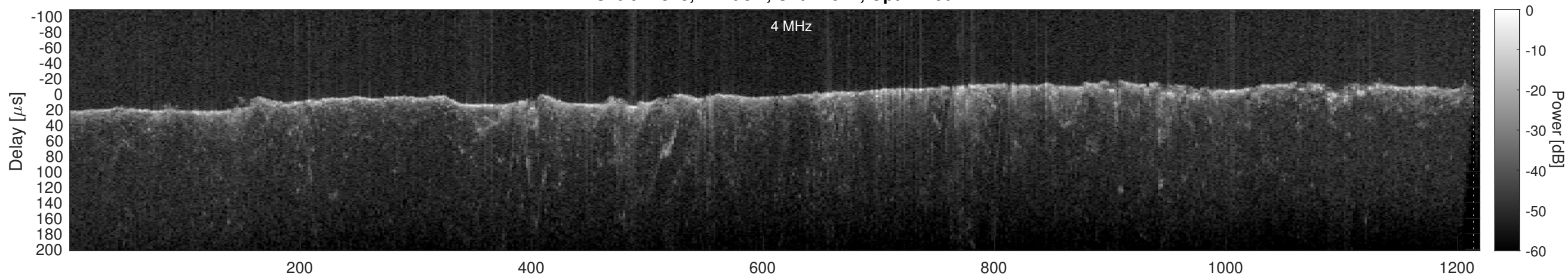
Orbit 11378, Cluttergram
