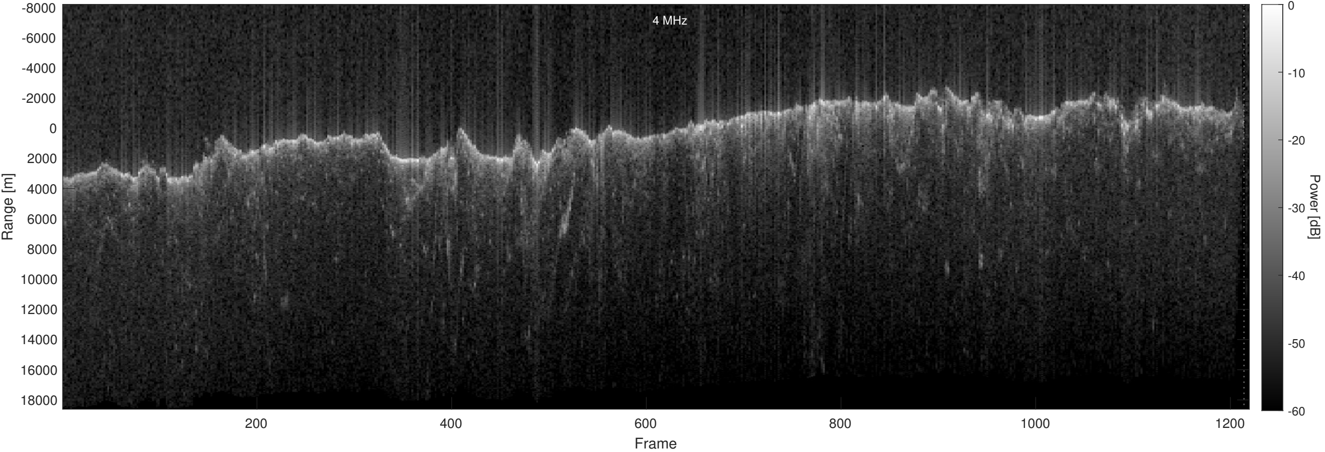
Orbit 11378, Optimized, No Window, Depth-Corrected, Channel 2
