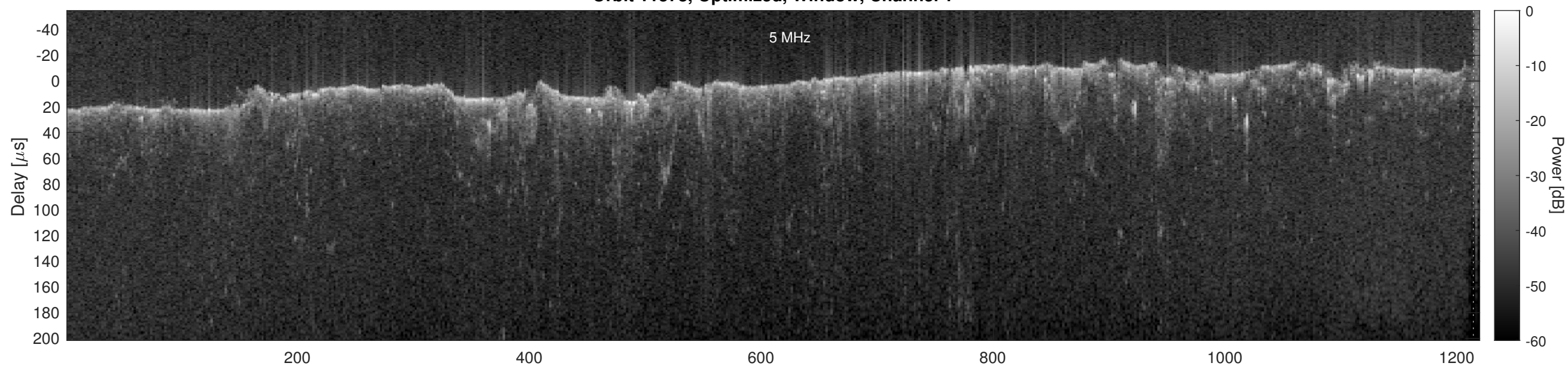
Orbit 11378, Optimized, Window, Channel 2
