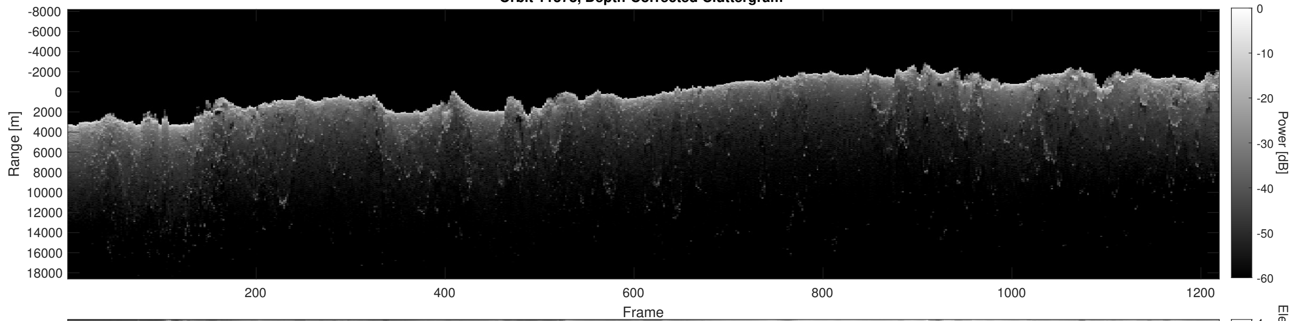
Orbit 11378, Depth-Corrected Cluttergram
