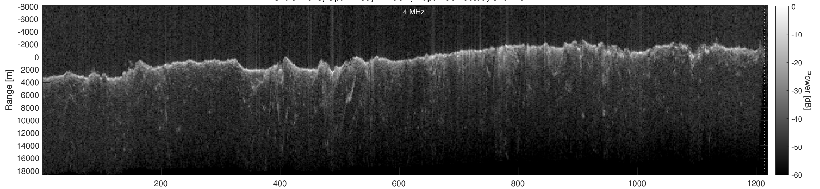
Orbit 11378, Depth-Corrected Cluttergram
