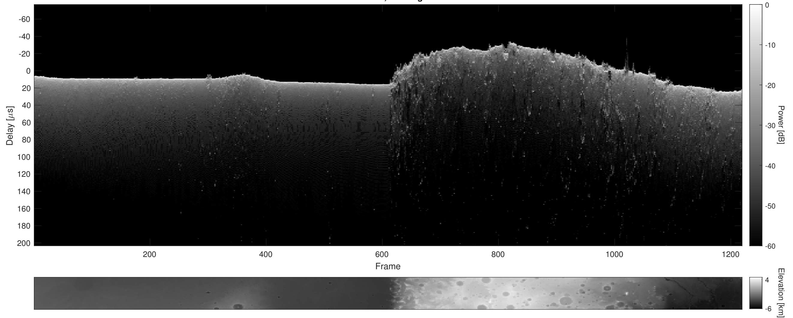
Orbit 11381, Cluttergram
