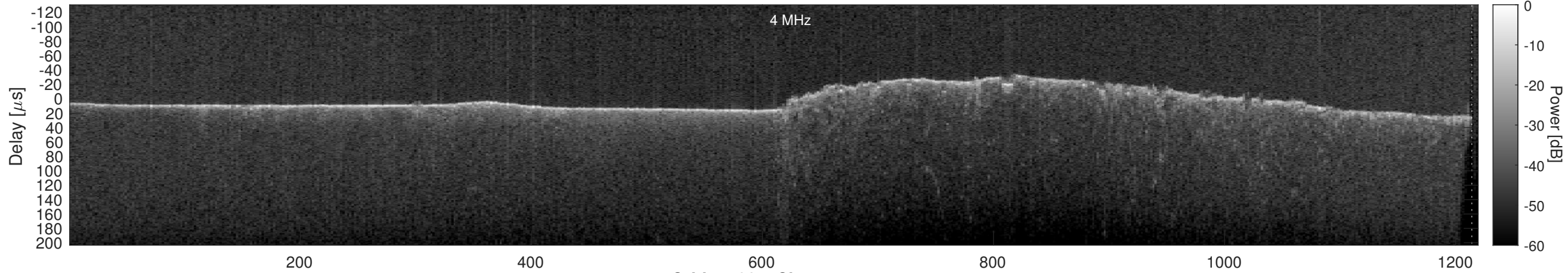
Orbit 11381, Cluttergram
