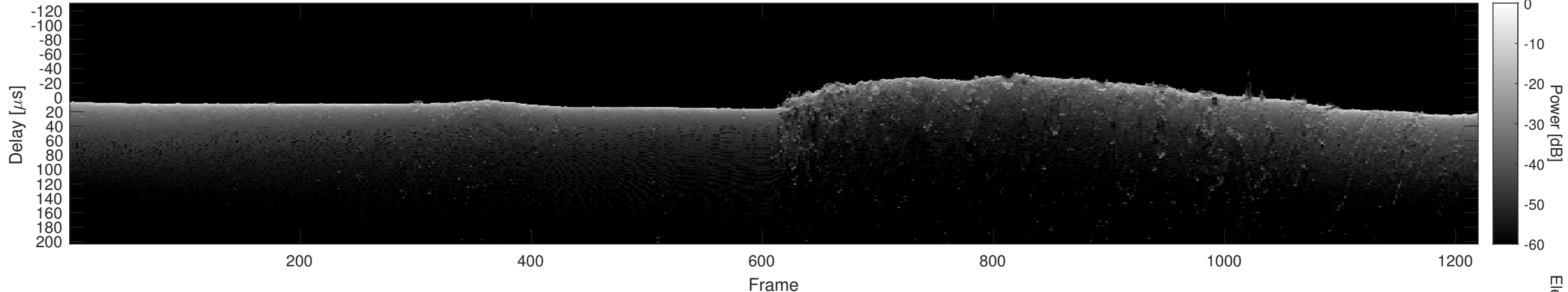
Orbit 11381, Cluttergram
