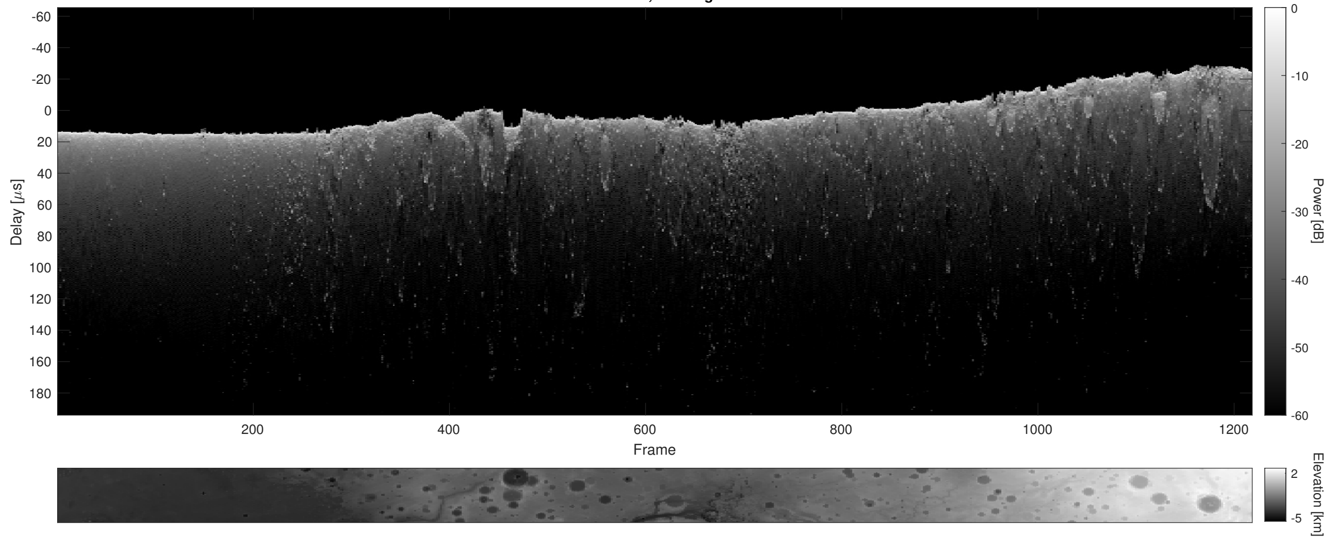
Orbit 11382, Cluttergram
