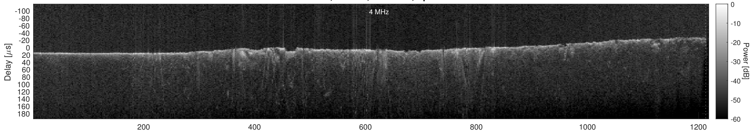
Orbit 11382, Cluttergram
