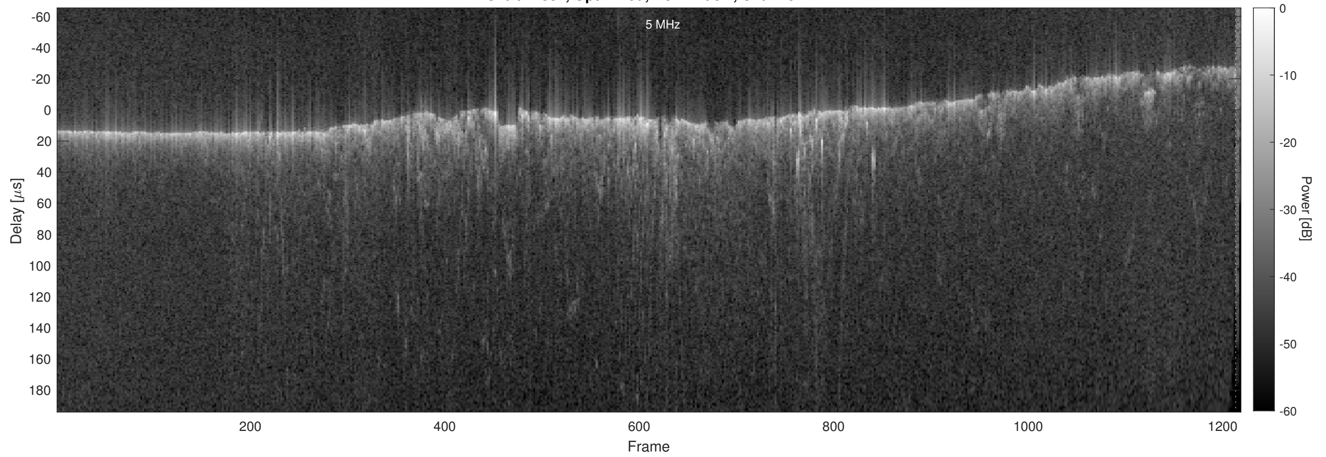
Orbit 11382, Optimized, No Window, Channel 2
