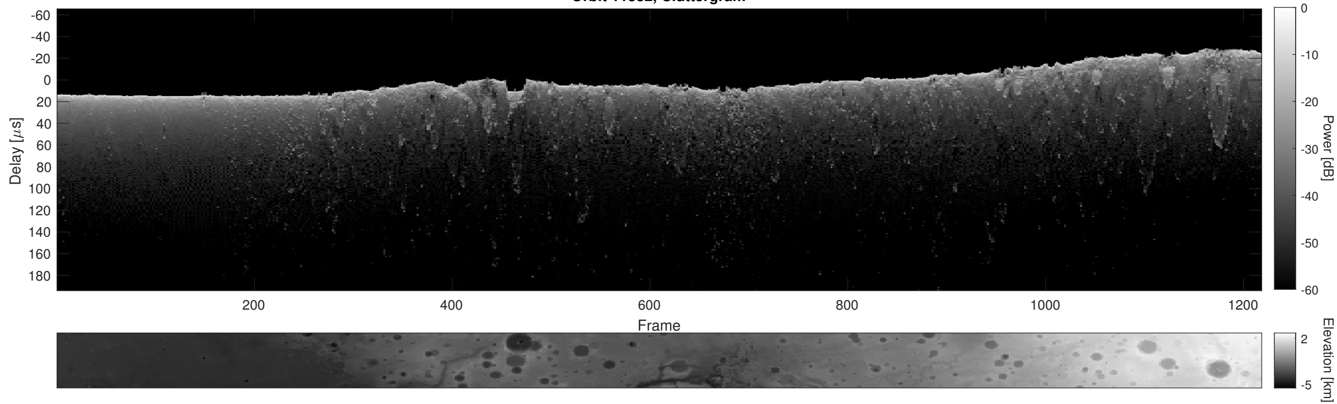
Orbit 11382, Cluttergram
