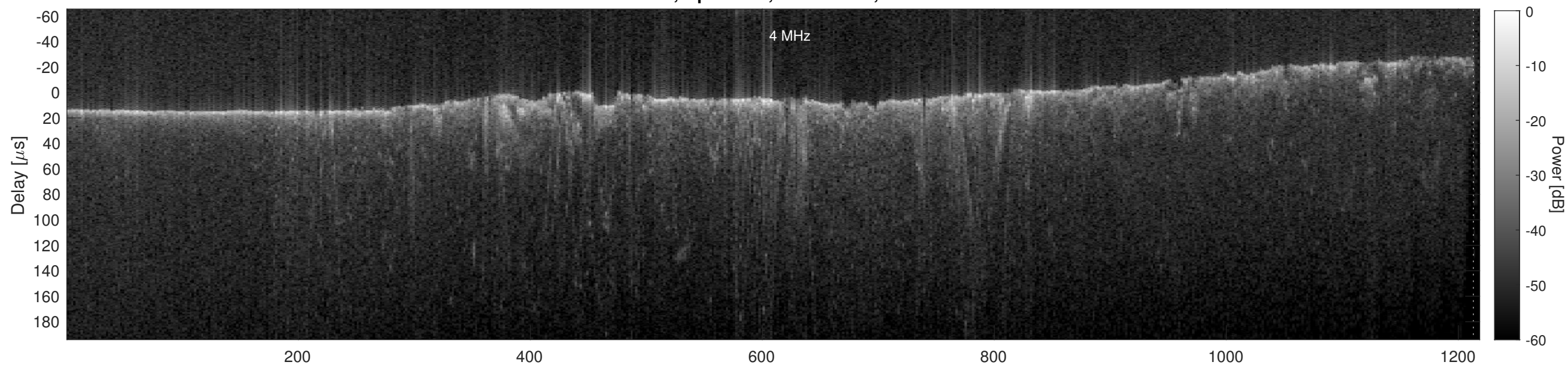
Orbit 11382, Cluttergram
