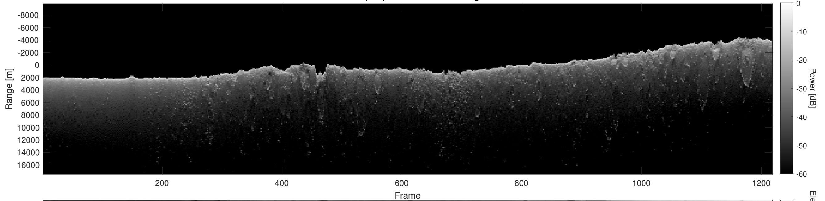
Orbit 11382, Depth-Corrected Cluttergram
