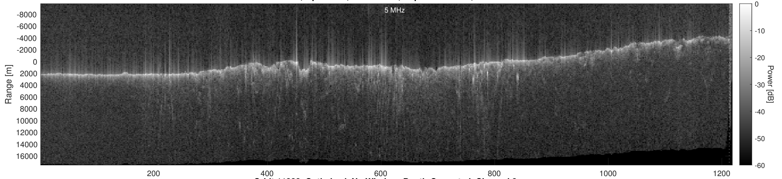
Orbit 11382, Optimized, No Window, Depth-Corrected, Channel 2
