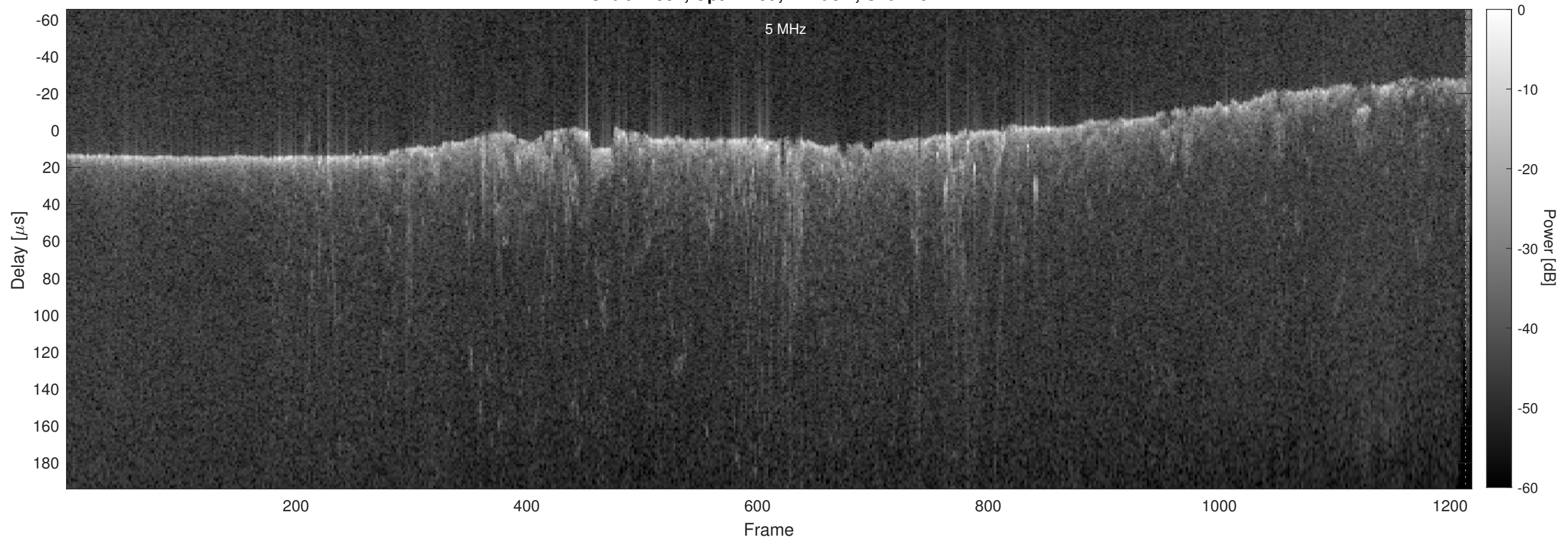
Orbit 11382, Optimized, Window, Channel 2
