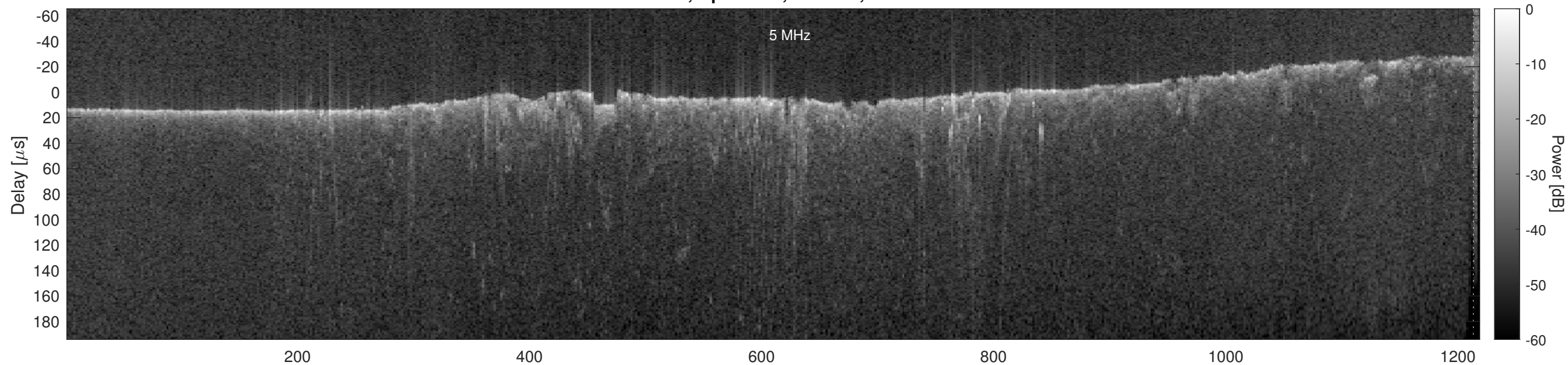
Orbit 11382, Optimized, Window, Channel 2
