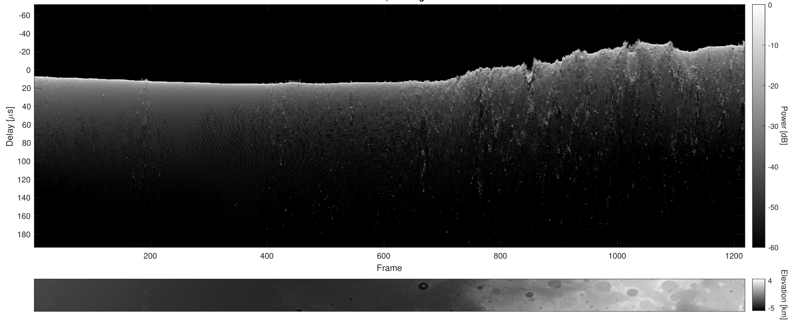
Orbit 11387, Cluttergram
