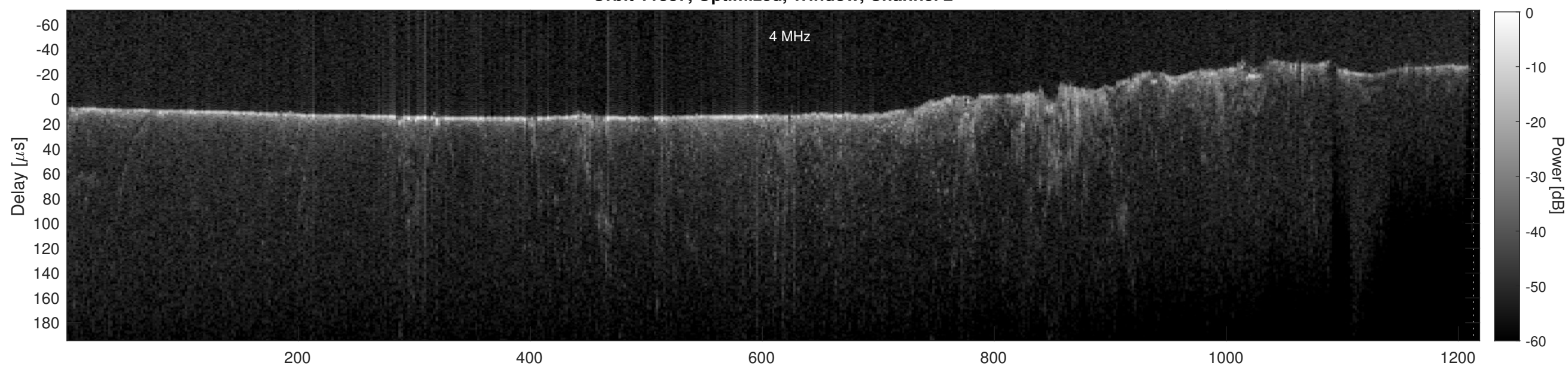
Orbit 11387, Cluttergram
