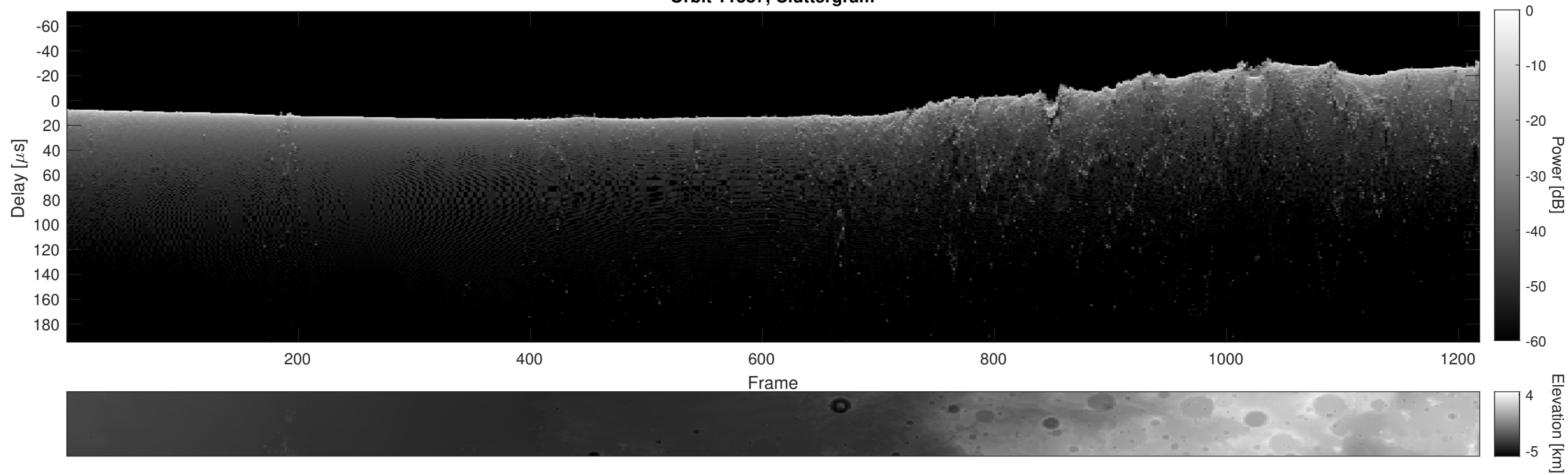
Orbit 11387, Cluttergram
