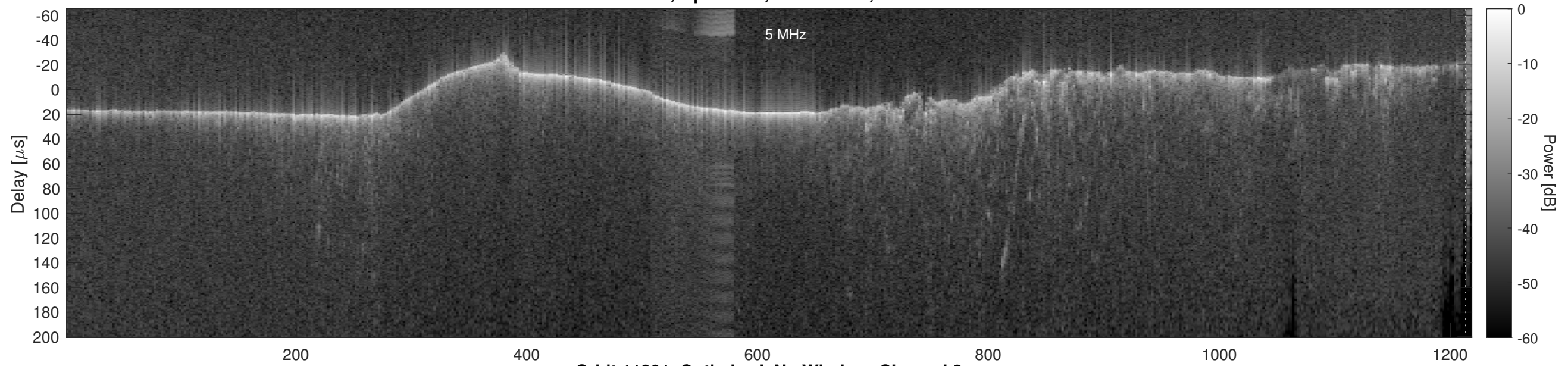
Orbit 11391, Optimized, No Window, Channel 2
