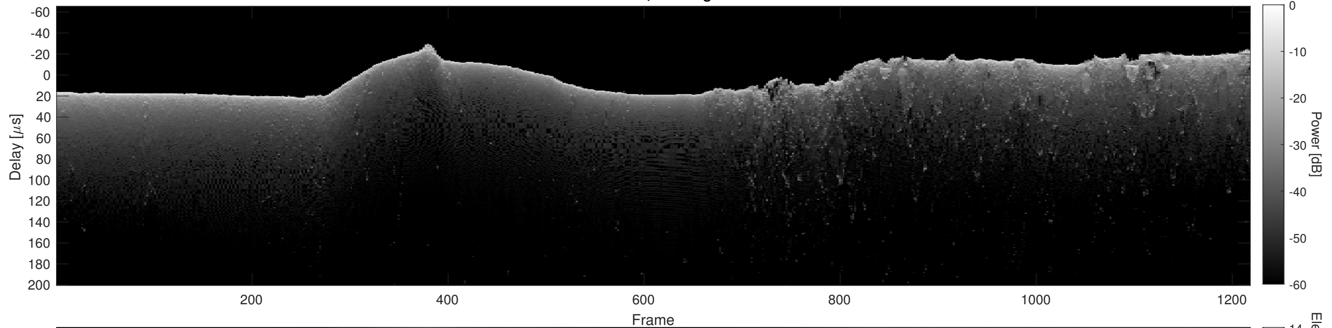
Orbit 11391, Cluttergram
