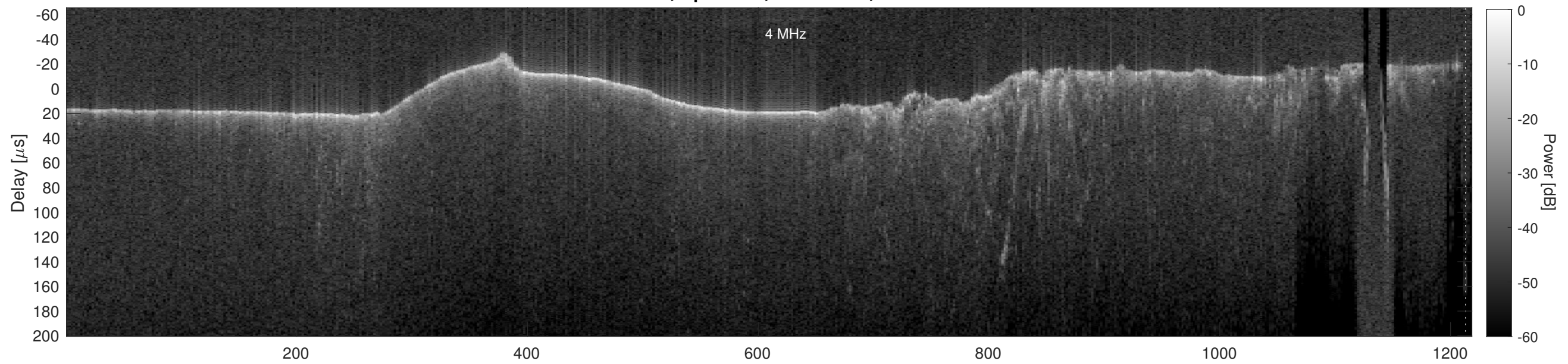
Orbit 11391, Cluttergram
