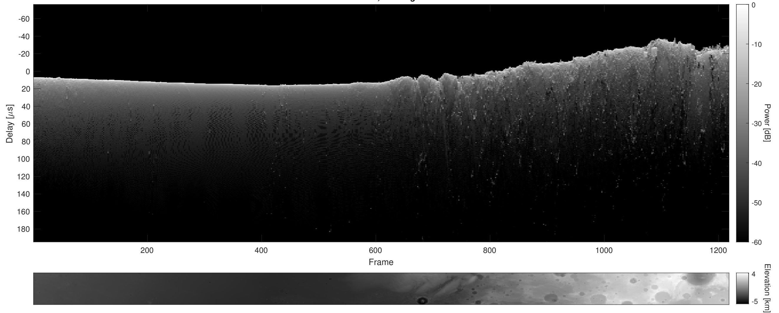
Orbit 11394, Cluttergram
