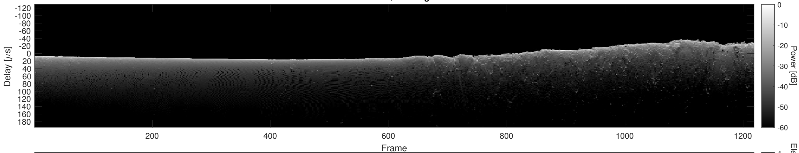
Orbit 11394, Cluttergram
