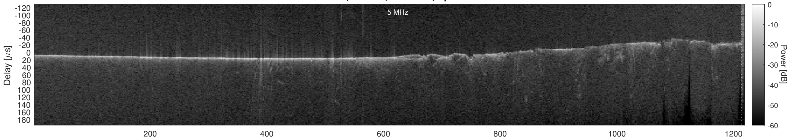
Orbit 11394, Cluttergram
