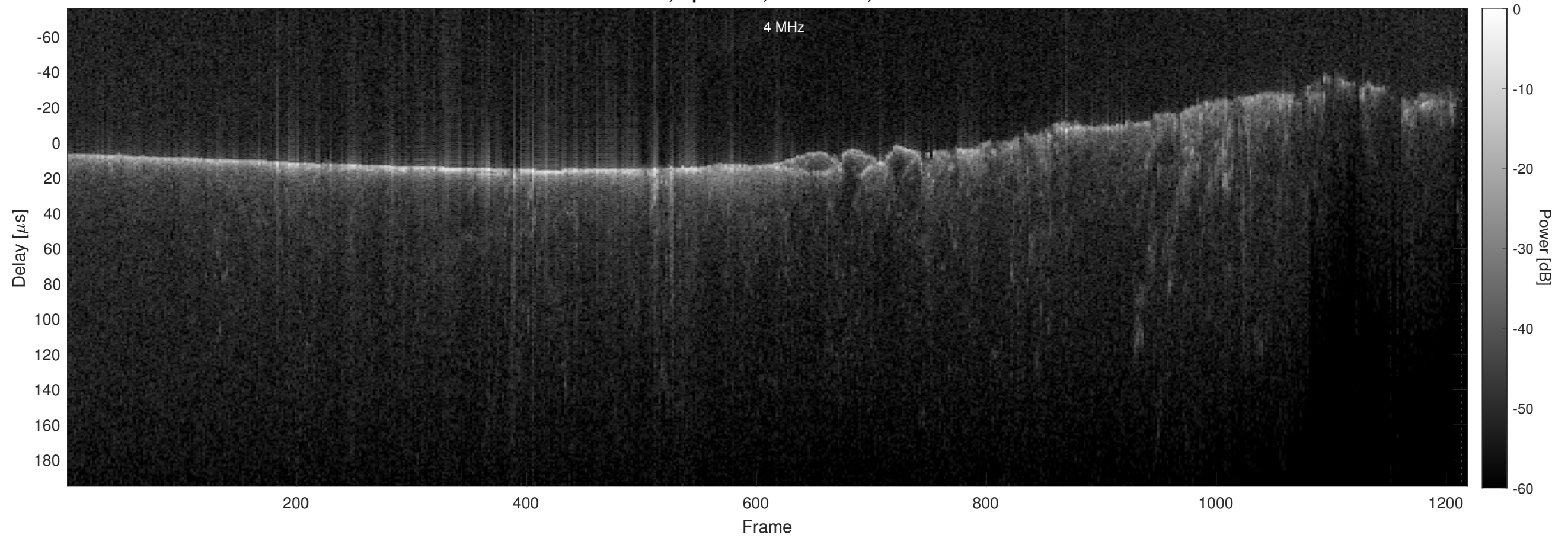
Orbit 11394, Optimized, No Window, Channel 2
