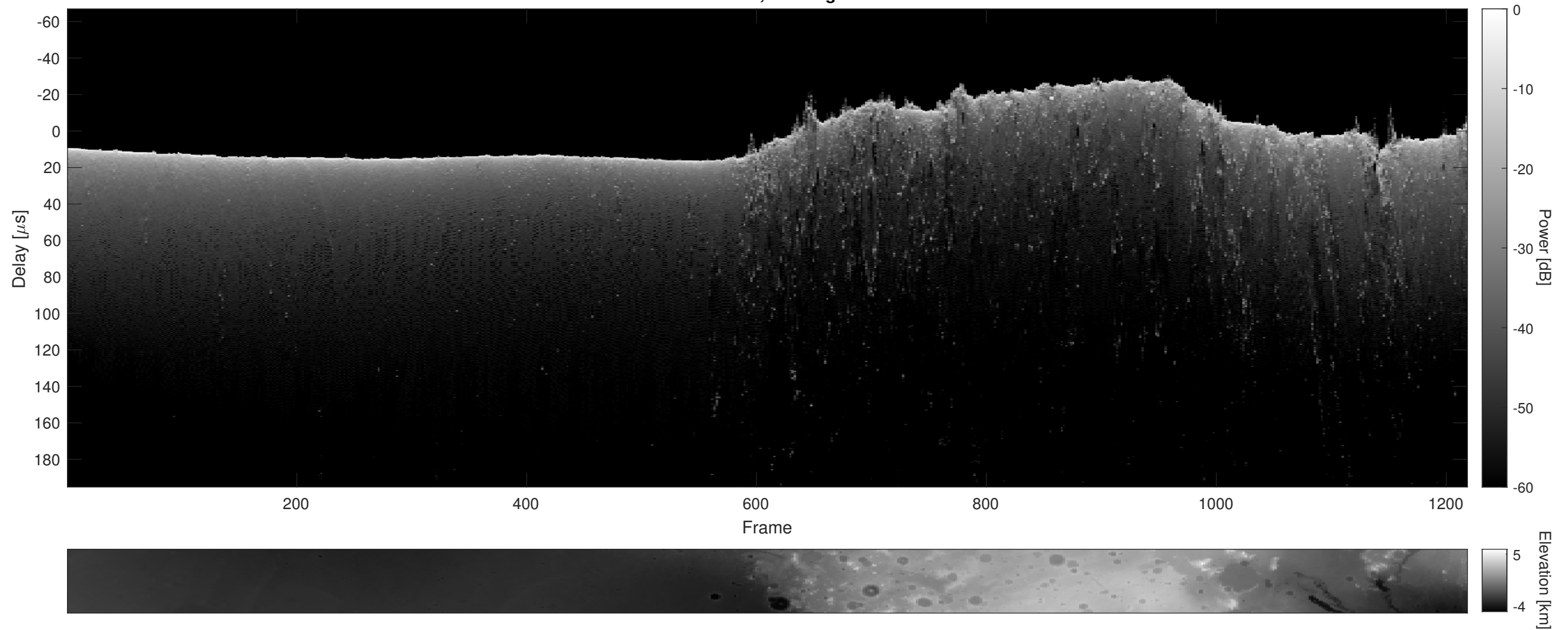
Orbit 11395, Cluttergram
