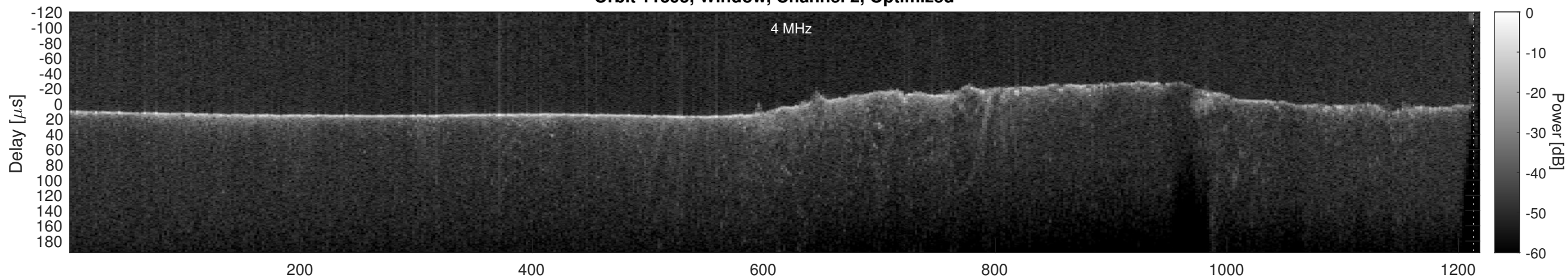
Orbit 11395, Cluttergram
