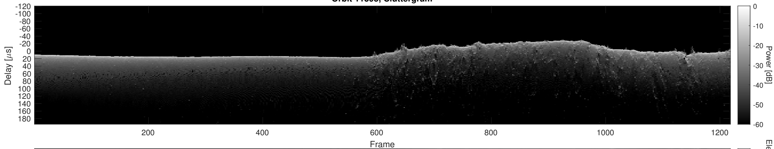
Orbit 11395, Cluttergram
