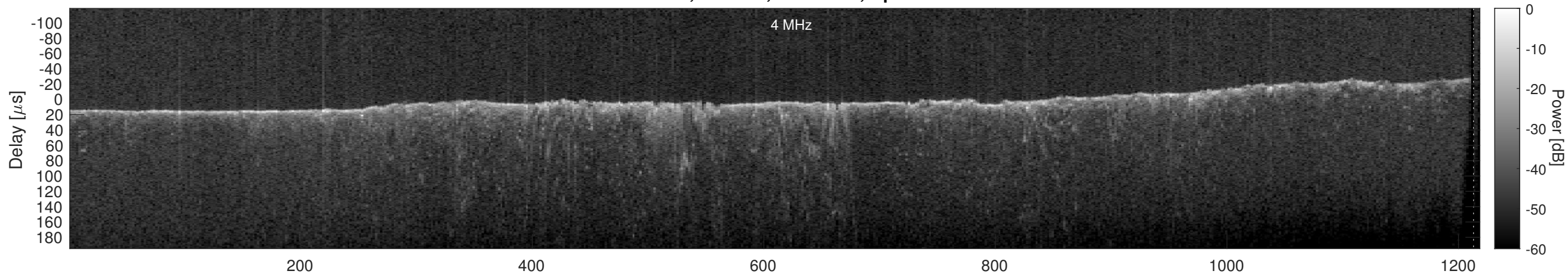
Orbit 11396, Cluttergram
