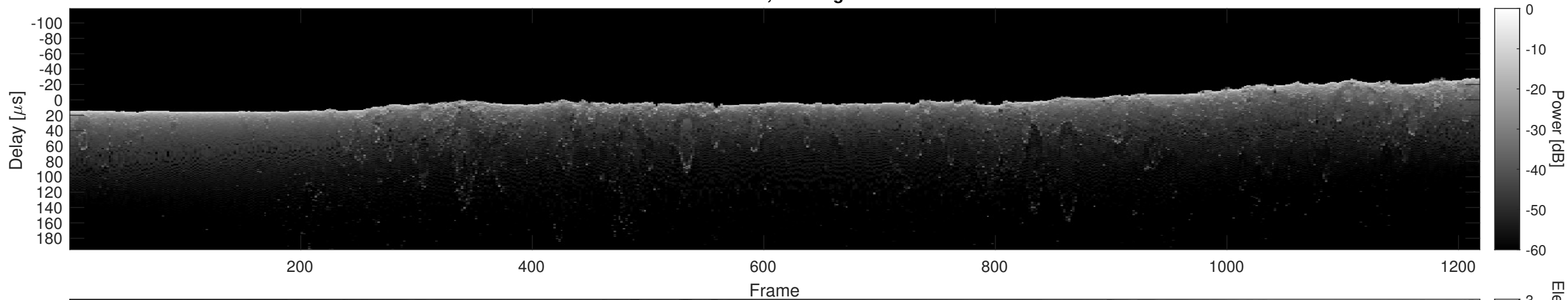
Orbit 11396, Cluttergram
