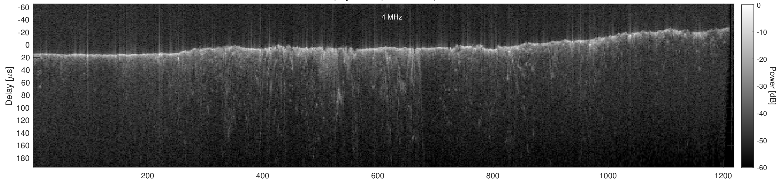
Orbit 11396, Cluttergram
