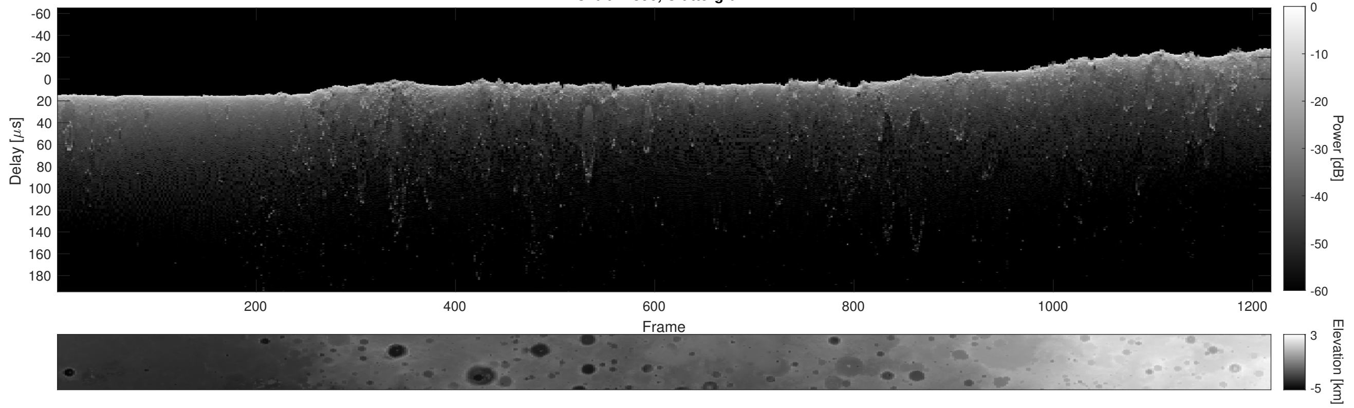
Orbit 11396, Cluttergram
