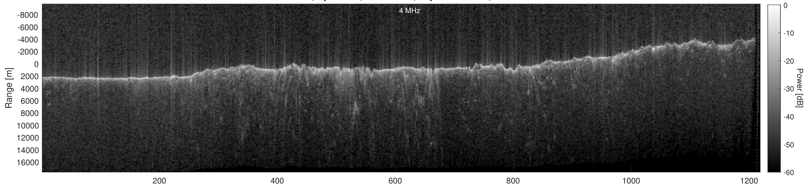
Orbit 11396, Depth-Corrected Cluttergram
