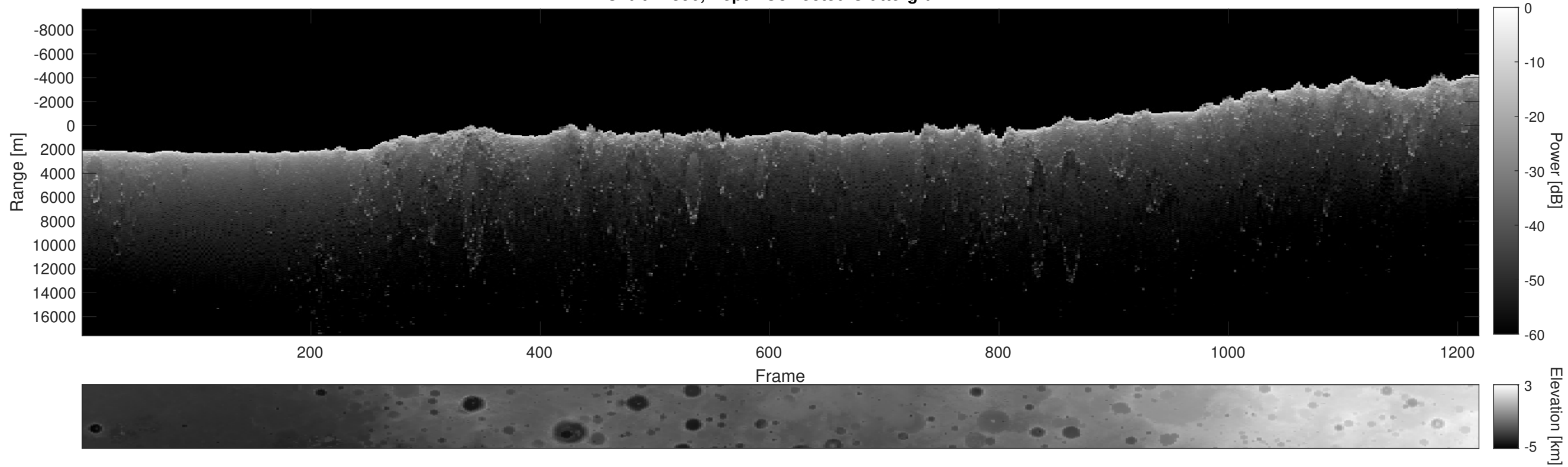
Orbit 11396, Depth-Corrected Cluttergram
