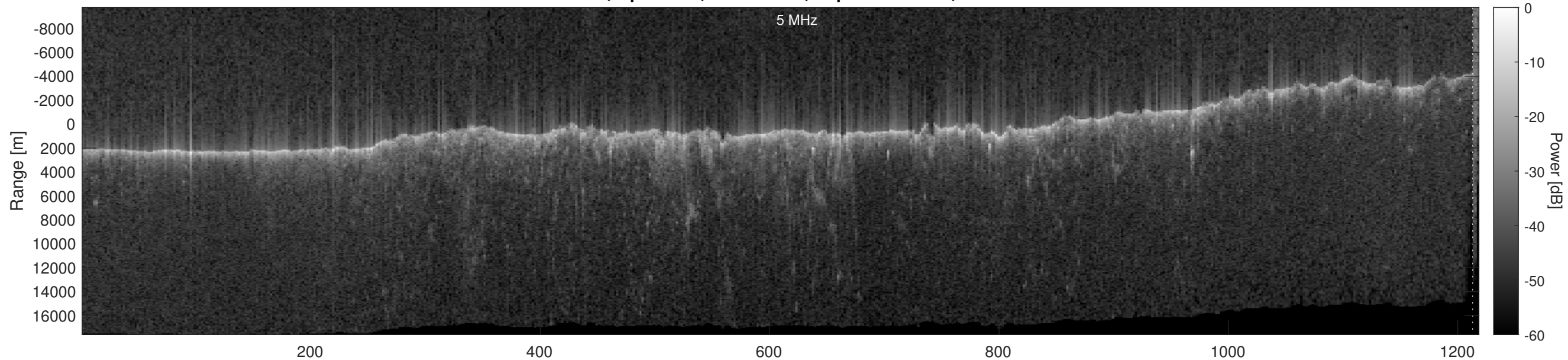
Orbit 11396, Optimized, No Window, Depth-Corrected, Channel 2
