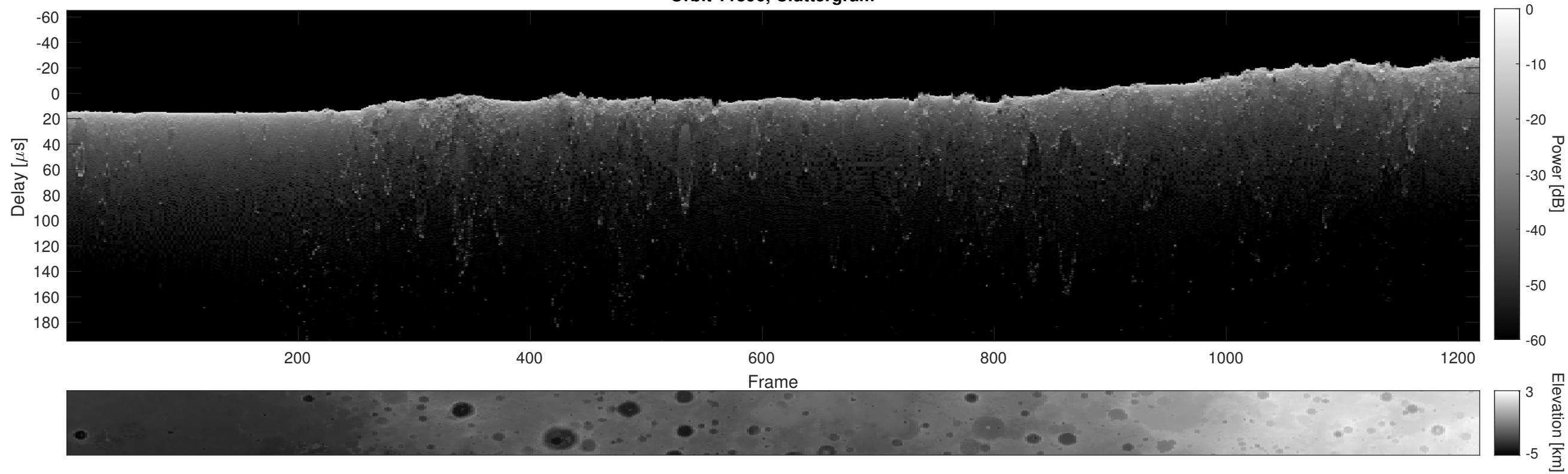
Orbit 11396, Cluttergram
