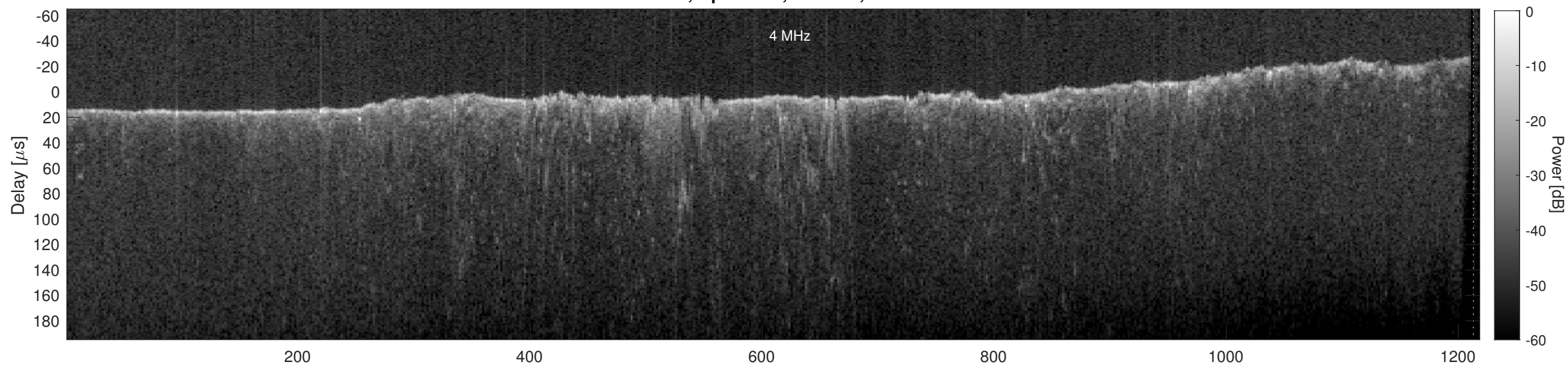
Orbit 11396, Cluttergram
